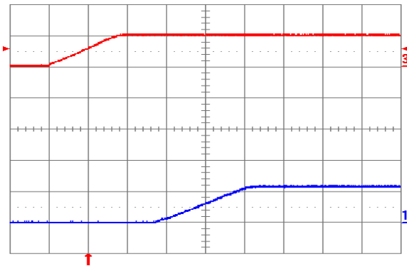
Fig. 1.2V.5: Turn-on transient (YNV05T10012) with application of V_{in} at full rated load current (resistive) and 47\mu\text{F} external capacitance at V_{in} = 5\text{V} . Top trace: V_{in} (5V/div.); Bottom trace: output voltage (1V/div.); Time scale: 2ms/div.
