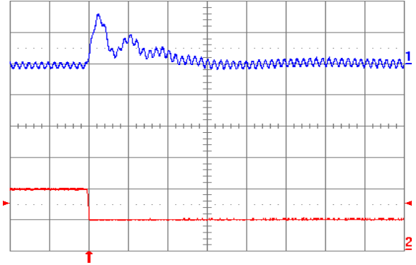
Fig. 3.3V.8: Output voltage response (YNV05T10033) to negative load current step change from 5A to 2.5A with slew rate of -5A/μs at Vin = 5V. Top trace: output voltage (100mV/div.); Bottom trace: load current (5A/div.). Co = 100μF ceramic + 1μF ceramic. Time scale: 20μs/div.
