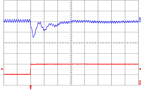
Fig. 3.3V.7: Output voltage response (YNV05T10033) to positive load current step change from 2.5A to 5A with slew rate of 5A/μs at Vin = 5V. Top trace: output voltage (100mV/div.); Bottom trace: load current (5A/div.). Co = 100μF ceramic + 1μF ceramic. Time scale: 20μs/div.
