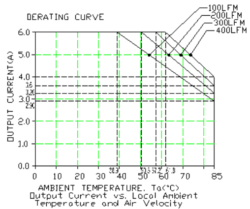
Figure 14. Vout = 5.5 V
