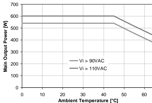
Figure 40. Thermal derating for PFE600-12-054RA
