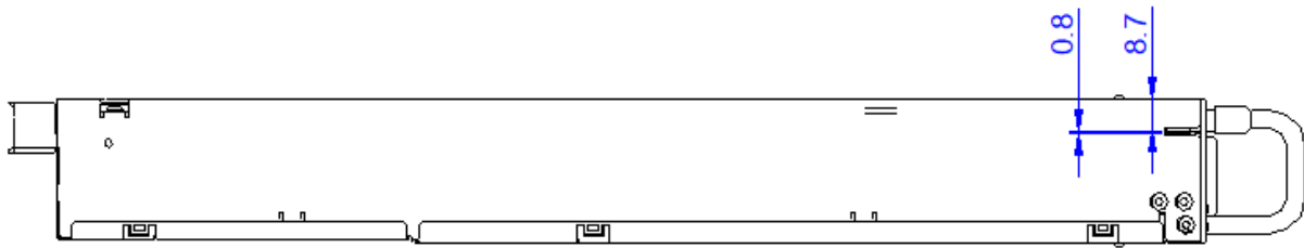
Figure 43. Side View 2
