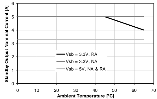
Figure 22. Temperature derating on V_{SB}
