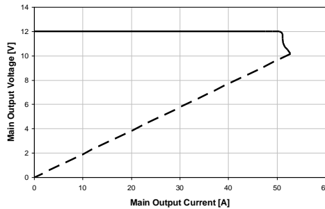
Figure 18. Current Limitation on V_1 ( V_i = 230 VAC)
