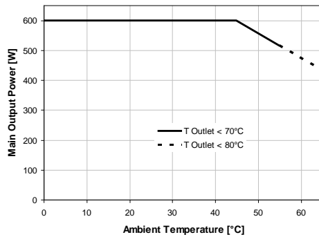
Figure 39. Thermal derating for PFE600-12-054NA
