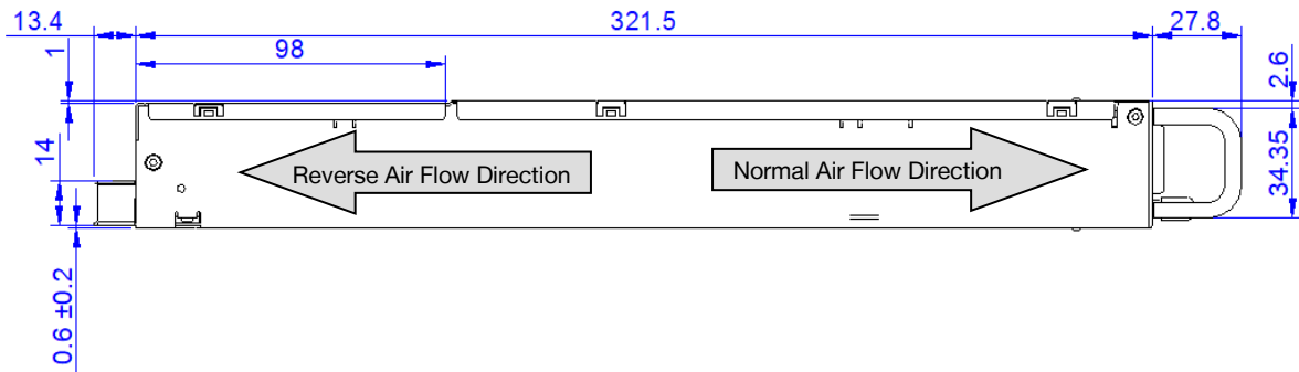
Figure 41. Side View 1
