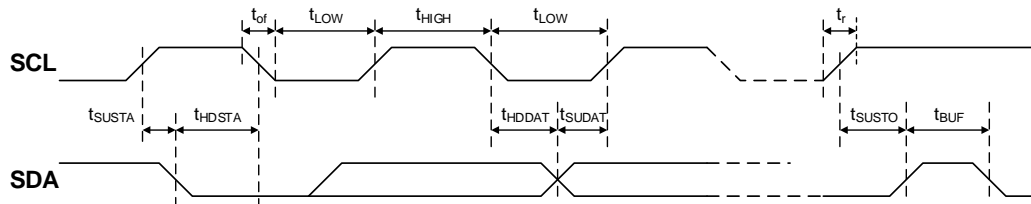
Figure 33. I 2 C / SMBus Timing
