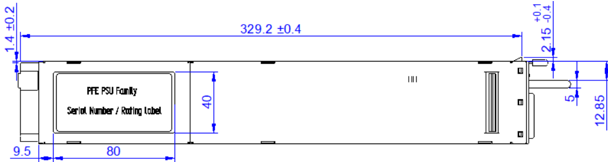
Figure 42. Top View
