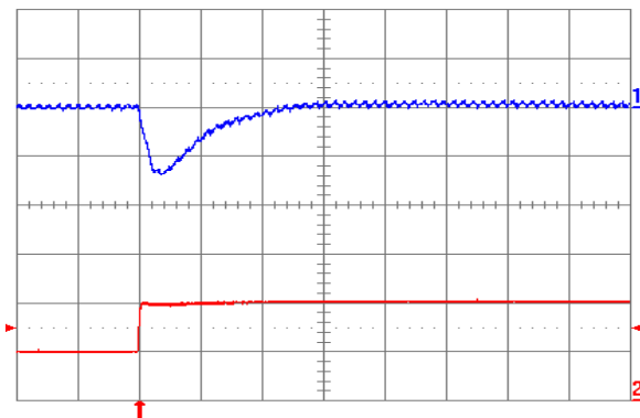
Fig. 2.5V.7: Output voltage response (YNV12T10025) to positive load current step change from 5 A to 10 A with slew rate of 5\ \text{A}/\mu\text{s} at V_{in} = 12\ \text{V} . Top trace: output voltage (100 mV/div.); Bottom trace: load current (5 A/div.). C_o = 100\ \mu\text{F} ceramic. Time scale: 20\ \mu\text{s}/\text{div} .
