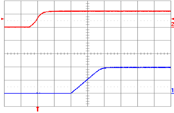
Fig. 1.0V.5: Turn-on transient (YNV12T10010) with application of V_{in} at full rated load current (resistive) and 100\ \mu\text{F} external capacitance at V_{in} = 12\ \text{V} . Top trace: V_{in} ( 10\ \text{V/div.} ); Bottom trace: output voltage ( 0.5\ \text{V/div.} ); Time scale: 2\ \text{ms/div.}
