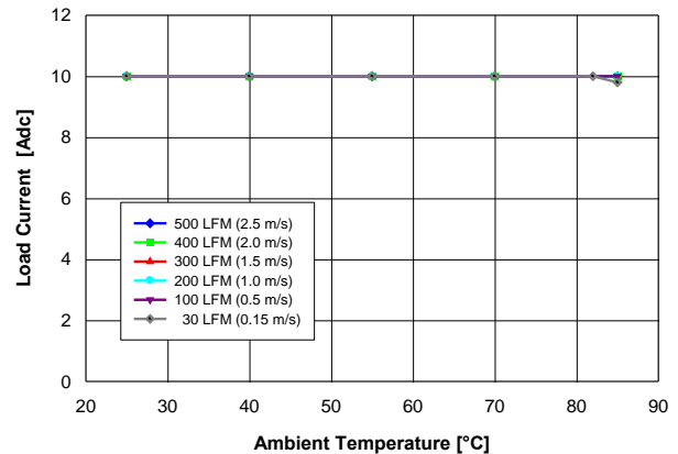
Fig. 1.5V.2: Available load current vs. ambient temperature and airflow rates for YNV12T10015 converter mounted horizontally with V_{in} = 12\ \text{V} , and maximum MOSFET temperature \leq 120\ ^\circ\text{C} .
