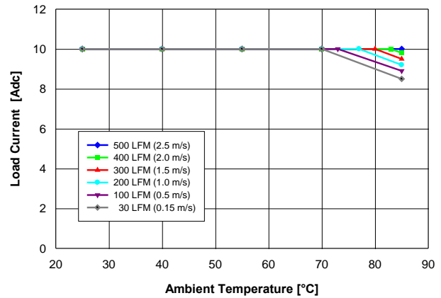
Fig. 5.0V.2: Available load current vs. ambient temperature and airflow rates for YNV12T10050 converter mounted horizontally with V_{in} = 12\text{ V} , and maximum MOSFET temperature \leq 120\text{ }^{\circ}\text{C} .
