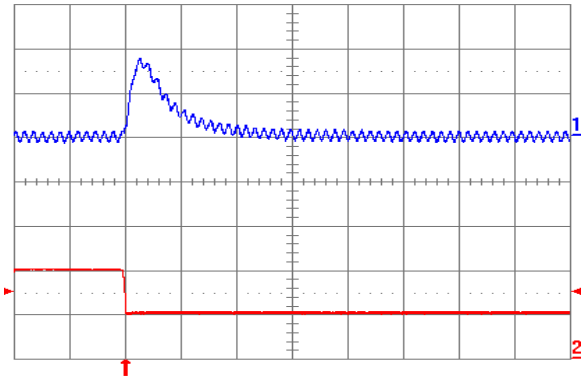
Fig. 5.0V.8: Output voltage response (YNV12T10050) to negative load current step change from 10 A to 5 A with slew rate of -5 A/μs at Vin = 12 V. Top trace: output voltage (100 mV/div.); Bottom trace: load current (5 A/div.). Co = 100 μF ceramic. Time scale: 20 μs/div.
