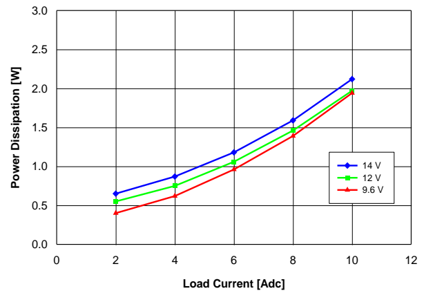
Fig. 1.2V.4: Power loss vs. load current and input voltage for YNV12T10012 converter mounted vertically with air flowing at a rate of 200 LFM (1 m/s) and T_a = 25\text{ }^{\circ}\text{C} .
