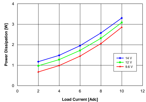
Fig. 5.0V.4: Power loss vs. load current and input voltage for YNV12T10050 converter mounted vertically with air flowing at a rate of 200 LFM (1 m/s) and T_a = 25\text{ }^{\circ}\text{C} .
