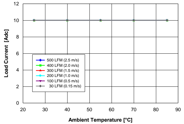
Fig. 1.0V.2: Available load current vs. ambient temperature and airflow rates for YNV12T10010 converter mounted horizontally with V_{in} = 12 V, and maximum MOSFET temperature \leq 120 °C.
