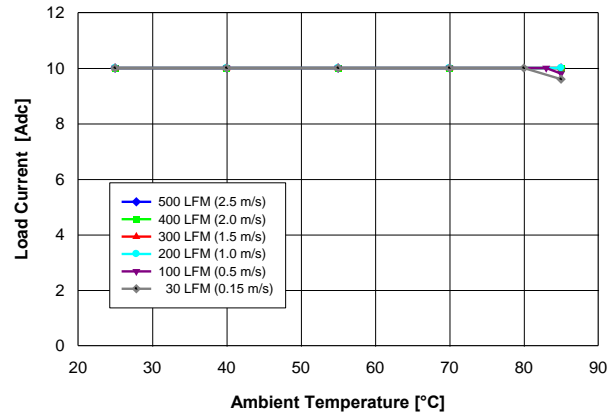
Fig. 1.8V.2: Available load current vs. ambient temperature and airflow rates for YNV12T10018 converter mounted horizontally with V_{in} = 12 V, and maximum MOSFET temperature \leq 120 °C.
