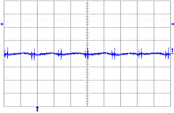
Fig. 1.0V.6: Output voltage ripple ( 20\ \text{mV/div.} ) at full rated load current into a resistive load with external capacitance 100\ \mu\text{F} ceramic and V_{in} = 12\ \text{V} (YNV12T10010). Time scale: 2\ \mu\text{s/div.}
