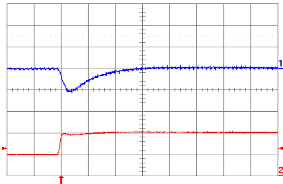
Fig. 1.0V.7: Output voltage response (YNV12T10010) to positive load current step change from 5\ \text{A} to 10\ \text{A} with slew rate of 5\ \text{A}/\mu\text{s} at V_{in} = 12\ \text{V} . Top trace: output voltage ( 100\ \text{mV/div.} ); Bottom trace: load current ( 5\ \text{A/div.} ). C_o = 100\ \mu\text{F} ceramic. Time scale: 20\ \mu\text{s/div.}
