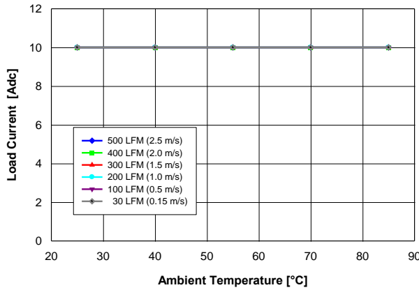
Fig. 1.0V.1: Available load current vs. ambient temperature and airflow rates for YNV12T10010 converter mounted vertically with V_{in} = 12 V, and maximum MOSFET temperature \leq 120 °C.
