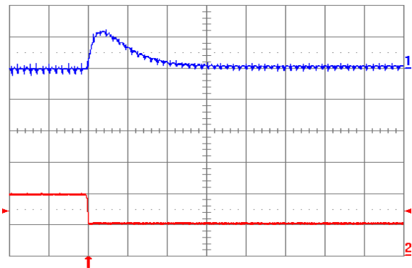
Fig. 1.5V.8: Output voltage response (YNV12T10015) to negative load current step change from 10 A to 5 A with slew rate of -5\ \text{A}/\mu\text{s} at V_{in} = 12\ \text{V} . Top trace: output voltage (100 mV/div.); Bottom trace: load current (5 A/div.). C_o = 100\ \mu\text{F} ceramic. Time scale: 20 \mu\text{s} /div.
