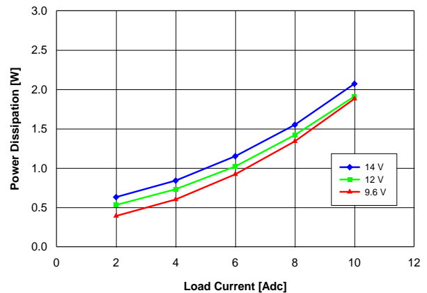
Fig. 1.0V.4: Power loss vs. load current and input voltage for YNV12T10010 converter mounted vertically with air flowing at a rate of 200 LFM (1 m/s) and T_a = 25 °C.
