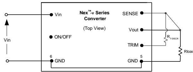
Fig. D: Configuration for programming output voltage.
