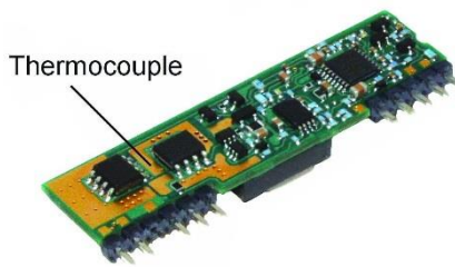
Fig. E: Location of the thermocouple for thermal testing
