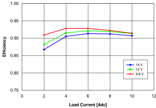
Fig. 2.5V.3: Efficiency vs. load current and input voltage for YNV12T10025 converter mounted vertically with air flowing at a rate of 200 LFM (1 m/s) and T_a = 25^\circ\text{C} .
