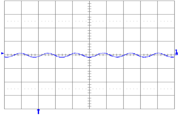
Fig. 1.8V.6: Output voltage ripple ( 20\ \text{mV/div.} ) at full rated load current into a resistive load with external capacitance 100\ \mu\text{F} ceramic and V_{in} = 12\ \text{V} (YNV12T10018). Time scale: 2\ \mu\text{s/div.}
