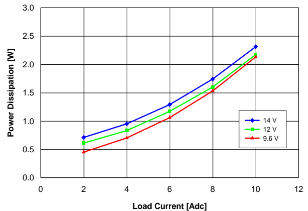
Fig. 1.8V.4: Power loss vs. load current and input voltage for YNV12T10018 converter mounted vertically with air flowing at a rate of 200 LFM (1 m/s) and T_a = 25 °C.
