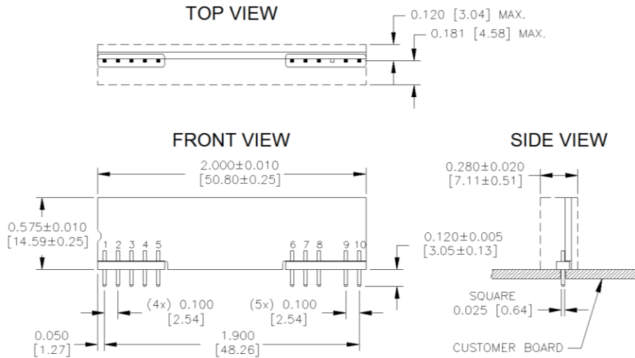
YNV12T100xy Pinout (Through-Hole - SIP)
