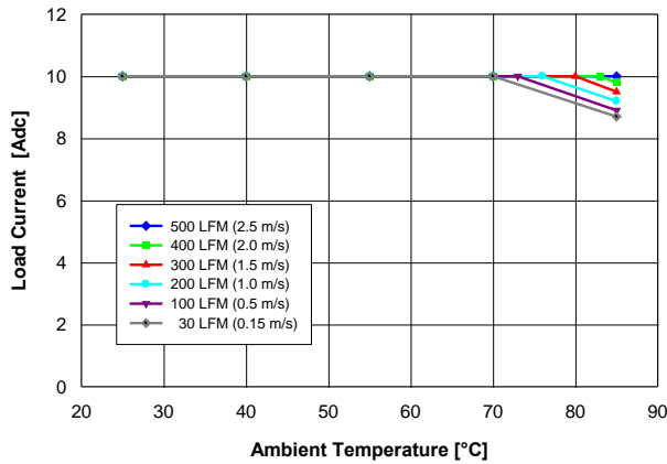
Fig. 5.0V.1: Available load current vs. ambient temperature and airflow rates for YNV12T10050 converter mounted vertically with V_{in} = 12\text{ V} , and maximum MOSFET temperature \leq 120\text{ }^{\circ}\text{C} .
