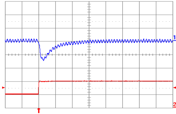
Fig. 5.0V.7: Output voltage response (YNV12T10050) to positive load current step change from 5 A to 10 A with slew rate of 5 A/μs at Vin = 12V. Top trace: output voltage (100 mV/div.); Bottom trace: load current (5 A/div.). Co = 100 μF ceramic. Time scale: 20 μs/div.
