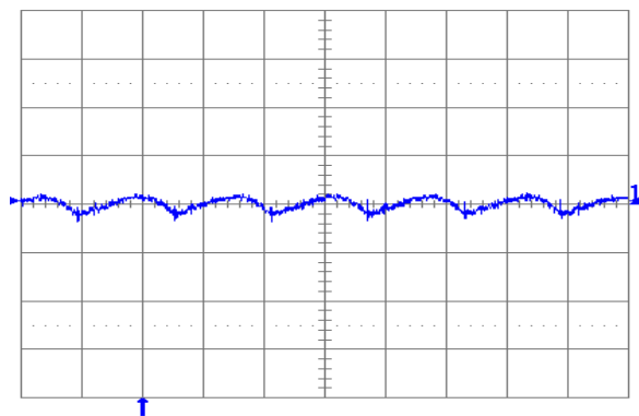
Fig. 2.0V.6: Output voltage ripple (20 mV/div.) at full rated load current into a resistive load with external capacitance 100\text{ }\mu\text{F} ceramic and V_{in} = 12\text{ V} (YNV12T10020). Time scale: 2 \mu\text{s} /div.
