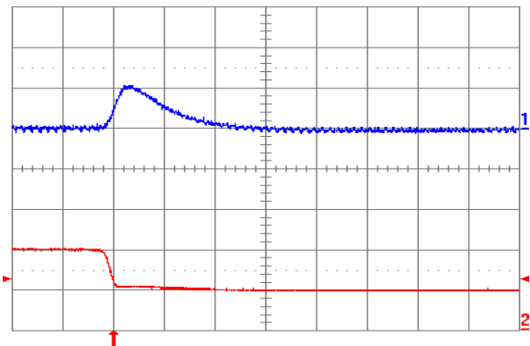
Fig. 1.0V.8: Output voltage response (YNV12T10010) to negative load current step change from 10\ \text{A} to 5\ \text{A} with slew rate of -5\ \text{A}/\mu\text{s} at V_{in} = 12\ \text{V} . Top trace: output voltage ( 100\ \text{mV/div.} ); Bottom trace: load current ( 5\ \text{A/div.} ). C_o = 100\ \mu\text{F} ceramic. Time scale: 20\ \mu\text{s/div.}
