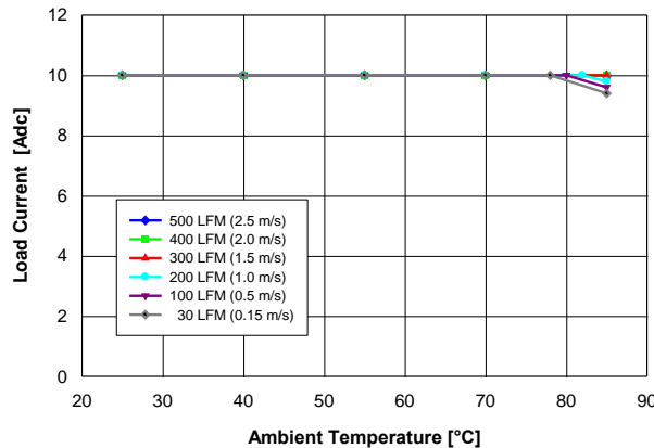
Fig. 2.5V.1: Available load current vs. ambient temperature and airflow rates for YNV12T10025 converter mounted vertically with V_{in} = 12\text{ V} , and maximum MOSFET temperature \leq 120\text{ }^\circ\text{C} .
