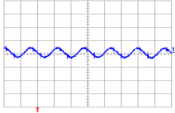
Fig. 3.3V.6: Output voltage ripple (20 mV/div.) at full rated load current into a resistive load with external capacitance 100 \mu\text{F} ceramic and V_{in} = 12\text{ V} (YNV12T10033). Time scale: 2 \mu\text{s} /div.
