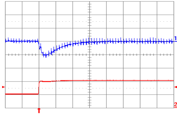
Fig. 1.2V.7: Output voltage response (YNV12T10012) to positive load current step change from 5 A to 10 A with slew rate of 5 A/μs at V_{in} = 12 V. Top trace: output voltage (100 mV/div.); Bottom trace: load current (5 A/div.). C_o = 100 μF ceramic. Time scale: 20 μs/div.
