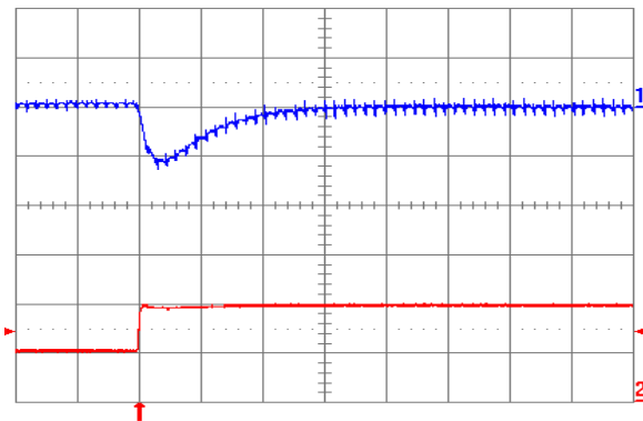
Fig. 1.5V.7: Output voltage response (YNV12T10015) to positive load current step change from 5 A to 10 A with slew rate of 5\ \text{A}/\mu\text{s} at V_{in} = 12\ \text{V} . Top trace: output voltage (100 mV/div.); Bottom trace: load current (5 A/div.). C_o = 100\ \mu\text{F} ceramic. Time scale: 20 \mu\text{s} /div.
