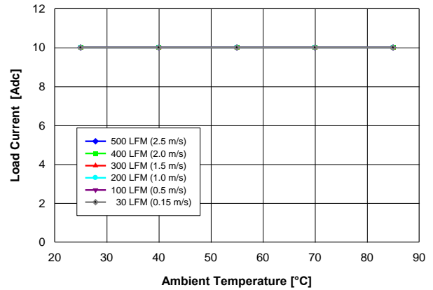
Fig. 1.2V.2: Available load current vs. ambient temperature and airflow rates for YNV12T10012 converter mounted horizontally with V_{in} = 12\text{ V} , and maximum MOSFET temperature \leq 120\text{ }^{\circ}\text{C} .
