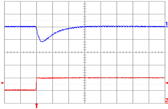
Fig. 2.0V.7: Output voltage response (YNV12T10020) to positive load current step change from 5 A to 10 A with slew rate of 5 A/μs at V_{in} = 12 V. Top trace: output voltage (100mV/div.); Bottom trace: load current (5 A/div.). C_o = 100 μF ceramic. Time scale: 20 μs/div.
