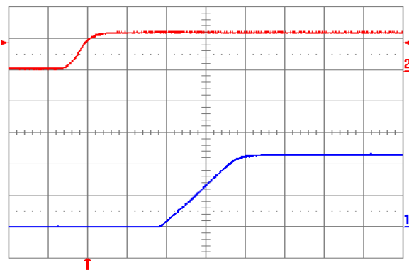
Fig. 1.2V.5: Turn-on transient (YNV12T10012) with application of V_{in} at full rated load current (resistive) and 100\text{ }\mu\text{F} external capacitance at V_{in} = 12\text{ V} . Top trace: V_{in} (10 V/div.); Bottom trace: output voltage (0.5 V/div.); Time scale: 2 ms/div.
