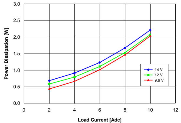
Fig. 1.5V.4: Power loss vs. load current and input voltage for YNV12T10015 converter mounted vertically with air flowing at a rate of 200 LFM (1 m/s) and T_a = 25^\circ\text{C} .
