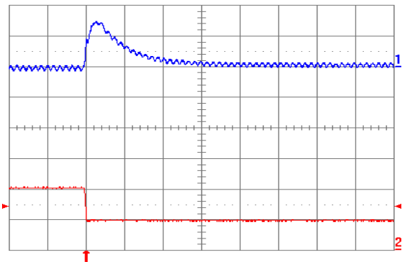
Fig. 3.3V.8: Output voltage response (YNV12T10033) to negative load current step change from 10 A to 5 A with slew rate of -5 A/ \mu\text{s} at V_{in} = 12\text{ V} . Top trace: output voltage (100 mV/div.); Bottom trace: load current (5 A/div.). C_o = 100\text{ }\mu\text{F} ceramic. Time scale: 20 \mu\text{s} /div.
