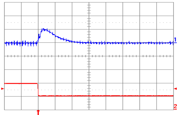
Fig. 1.8V.8: Output voltage response (YNV12T10018) to negative load current step change from 10\ \text{A} to 5\ \text{A} with slew rate of -5\ \text{A}/\mu\text{s} at V_{in} = 12\ \text{V} . Top trace: output voltage ( 100\ \text{mV/div.} ); Bottom trace: load current ( 5\ \text{A/div.} ). C_o = 100\ \mu\text{F} ceramic. Time scale: 20\ \mu\text{s/div.}
