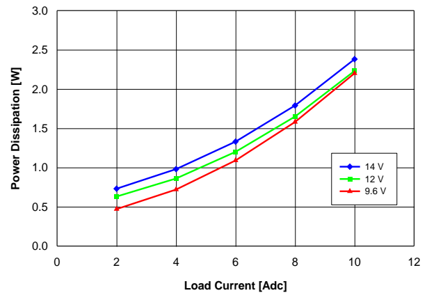
Fig. 2.0V.4: Power loss vs. load current and input voltage for YNV12T10020 converter mounted vertically with air flowing at a rate of 200 LFM (1 m/s) and T_a = 25\text{ }^{\circ}\text{C} .
