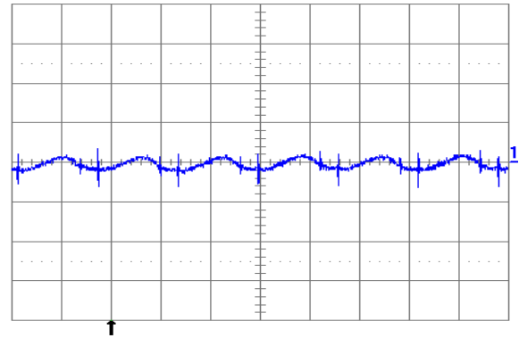
Fig. 2.5V.6: Output voltage ripple (20 mV/div.) at full rated load current into a resistive load with external capacitance 100\ \mu\text{F} ceramic and V_{in} = 12\ \text{V} (YNV12T10025). Time scale: 2\ \mu\text{s}/\text{div} .
