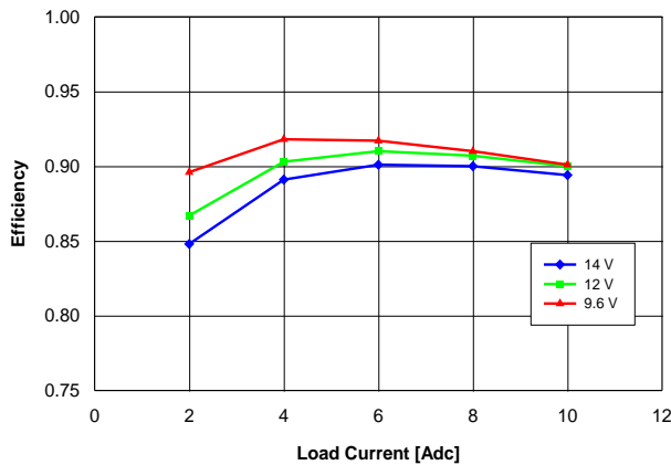
Fig. 2.0V.3: Efficiency vs. load current and input voltage for YNV12T10020 converter mounted vertically with air flowing at a rate of 200 LFM (1 m/s) and T_a = 25\text{ }^{\circ}\text{C} .
