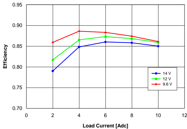
Fig. 1.2V.3: Efficiency vs. load current and input voltage for YNV12T10012 converter mounted vertically with air flowing at a rate of 200 LFM (1 m/s) and T_a = 25\text{ }^{\circ}\text{C} .
