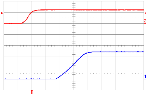
Fig. 2.5V.5: Turn-on transient (YNV12T10025) with application of V_{in} at full rated load current (resistive) and 100\ \mu\text{F} external capacitance at V_{in} = 12\ \text{V} . Top trace: V_{in} (10 V/div.); Bottom trace: output voltage (1 V/div.); Time scale: 2 ms/div.
