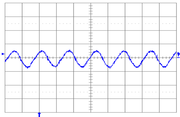
Fig. 5.0V.6: Output voltage ripple (20 mV/div.) at full rated load current into a resistive load with external capacitance 100 \mu\text{F} ceramic and V_{in} = 12\text{ V} (YNV12T10050). Time scale: 2 \mu\text{s} /div.
