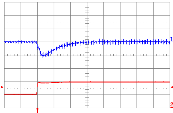
Fig. 1.8V.7: Output voltage response (YNV12T10018) to positive load current step change from 5\ \text{A} to 10\ \text{A} with slew rate of 5\ \text{A}/\mu\text{s} at V_{in} = 12\ \text{V} . Top trace: output voltage ( 100\ \text{mV/div.} ); Bottom trace: load current ( 5\ \text{A/div.} ). C_o = 100\ \mu\text{F} ceramic. Time scale: 20\ \mu\text{s/div.}
