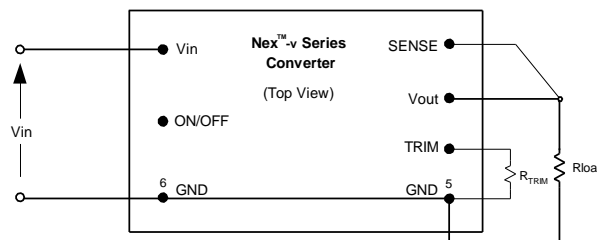
Fig. C: Configuration for increasing output voltage.
