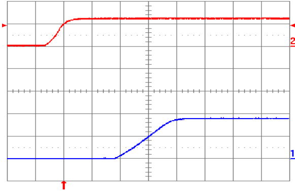
Fig. 1.8V.5: Turn-on transient (YNV12T10018) with application of V_{in} at full rated load current (resistive) and 100\ \mu\text{F} external capacitance at V_{in} = 12\ \text{V} . Top trace: V_{in} ( 10\ \text{V/div.} ); Bottom trace: output voltage ( 1\ \text{V/div.} ); Time scale: 2\ \text{ms/div.}
