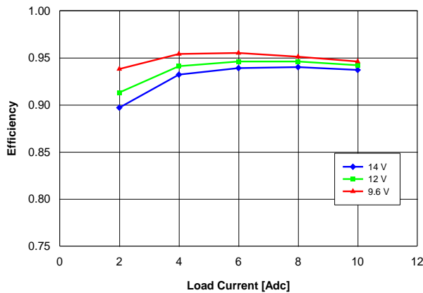
Fig. 5.0V.3: Efficiency vs. load current and input voltage for YNV12T10050 converter mounted vertically with air flowing at a rate of 200 LFM (1 m/s) and T_a = 25\text{ }^{\circ}\text{C} .
