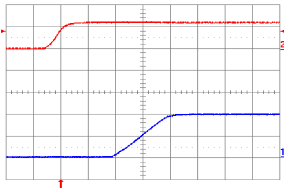
Fig. 2.0V.5: Turn-on transient (YNV12T10020) with application of V_{in} at full rated load current (resistive) and 100\text{ }\mu\text{F} external capacitance at V_{in} = 12\text{ V} . Top trace: V_{in} (10 V/div.); Bottom trace: output voltage (1 V/div.); Time scale: 2 ms/div.
