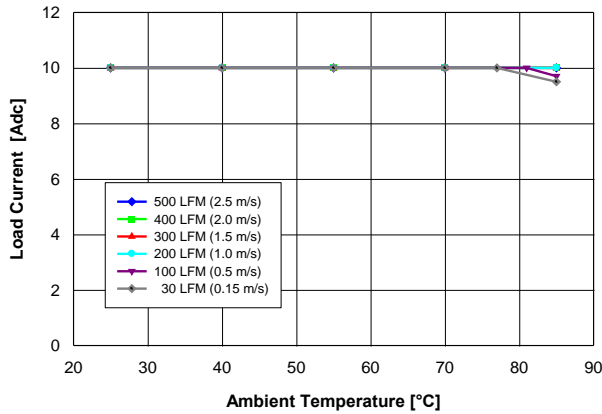
Fig. 2.0V.1: Available load current vs. ambient temperature and airflow rates for YNV12T10020 converter mounted vertically with V_{in} = 12\text{ V} , and maximum MOSFET temperature \leq 120\text{ }^{\circ}\text{C} .
