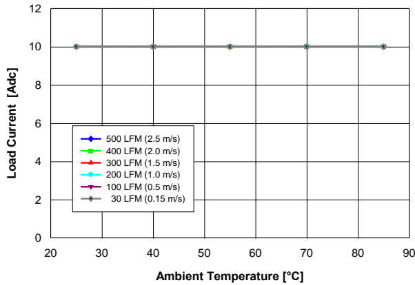
Fig. 1.2V.1: Available load current vs. ambient temperature and airflow rates for YNV12T10012 converter mounted vertically with V_{in} = 12\text{ V} , and maximum MOSFET temperature \leq 120\text{ }^{\circ}\text{C} .
