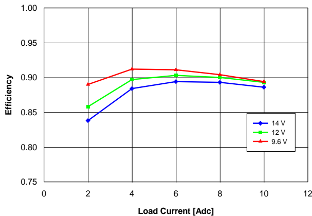
Fig. 1.8V.3: Efficiency vs. load current and input voltage for YNV12T10018 converter mounted vertically with air flowing at a rate of 200 LFM (1 m/s) and T_a = 25 °C.
