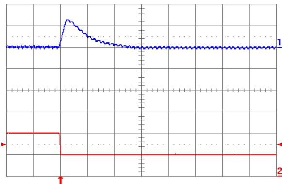
Fig. 2.5V.8: Output voltage response (YNV12T10025) to negative load current step change from 10 A to 5 A with slew rate of -5\ \text{A}/\mu\text{s} at V_{in} = 12\ \text{V} . Top trace: output voltage (100 mV/div.); Bottom trace: load current (5 A/div.). C_o = 100\ \mu\text{F} ceramic. Time scale: 20\ \mu\text{s}/\text{div} .
