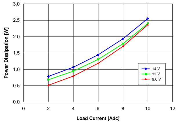
Fig. 2.5V.4: Power loss vs. load current and input voltage for YNV12T10025 converter mounted vertically with air flowing at a rate of 200 LFM (1 m/s) and T_a = 25^\circ\text{C} .
