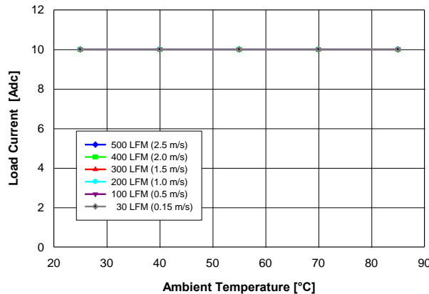
Fig. 1.5V.1: Available load current vs. ambient temperature and airflow rates for YNV12T10015 converter mounted vertically with V_{in} = 12\ \text{V} , and maximum MOSFET temperature \leq 120\ ^\circ\text{C} .
