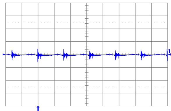
Fig. 1.2V.6: Output voltage ripple (20mV/div.) at full rated load current into a resistive load with external capacitance 100\text{ }\mu\text{F} ceramic and V_{in} = 12\text{ V} (YNV12T10012). Time scale: 2 \mu\text{s} /div.
