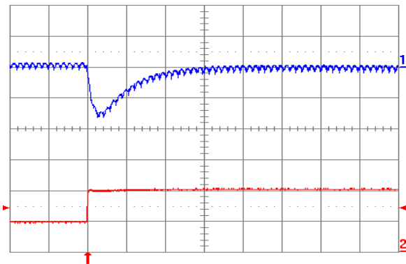
Fig. 3.3V.7: Output voltage response (YNV12T10033) to positive load current step change from 5 A to 10 A with slew rate of 5 A/ \mu\text{s} at V_{in} = 12\text{ V} . Top trace: output voltage (100 mV/div.); Bottom trace: load current (5 A/div.). C_o = 100\text{ }\mu\text{F} ceramic. Time scale: 20 \mu\text{s} /div.
