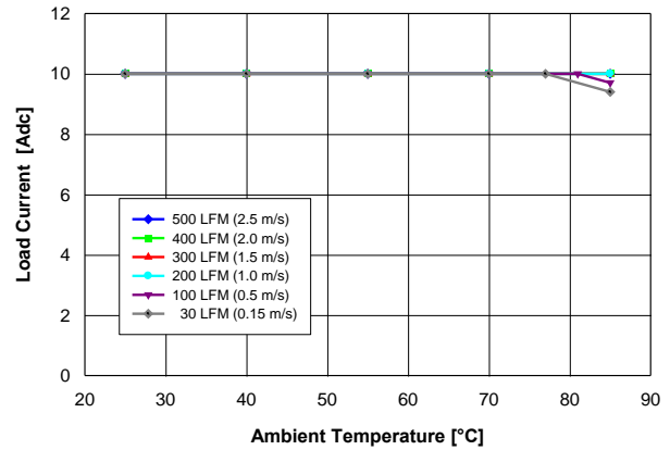
Fig. 2.0V.2: Available load current vs. ambient temperature and airflow rates for YNV12T10020 converter mounted horizontally with V_{in} = 12\text{ V} , and maximum MOSFET temperature \leq 120\text{ }^{\circ}\text{C} .
