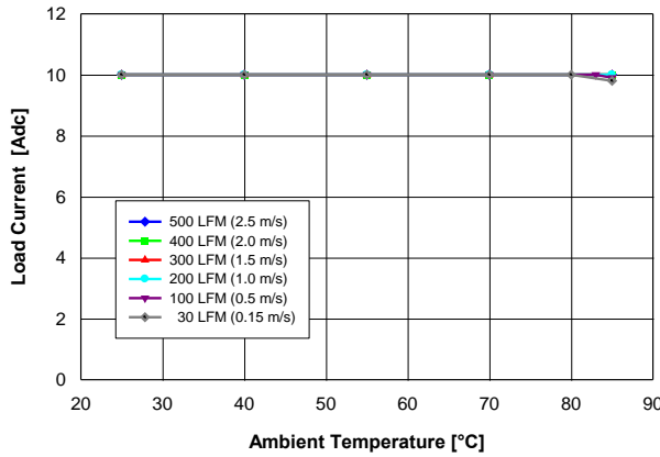
Fig. 1.8V.1: Available load current vs. ambient temperature and airflow rates for YNV12T10018 converter mounted vertically with V_{in} = 12 V, and maximum MOSFET temperature \leq 120 °C.
