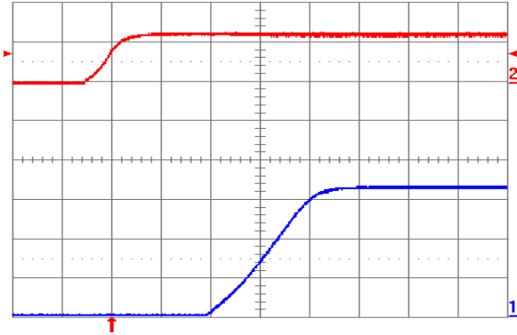
Fig. 3.3V.5: Turn-on transient (YNV12T10033) with application of V_{in} at full rated load current (resistive) and 100 \mu\text{F} external capacitance at V_{in} = 12\text{ V} . Top trace: V_{in} (10 V/div.); Bottom trace: output voltage (1 V/div.); Time scale: 2 ms/div.
