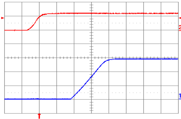
Fig. 1.5V.5: Turn-on transient (YNV12T10015) with application of V_{in} at full rated load current (resistive) and 100\ \mu\text{F} external capacitance at V_{in} = 12\ \text{V} . Top trace: V_{in} (10 V/div.); Bottom trace: output voltage (0.5 V/div.); Time scale: 2 ms/div.
