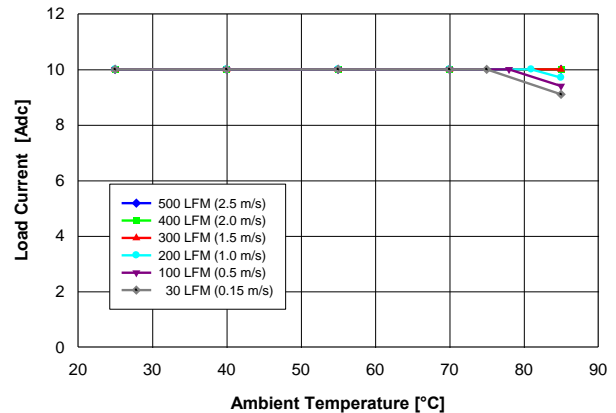
Fig. 2.5V.2: Available load current vs. ambient temperature and airflow rates for YNV12T10025 converter mounted horizontally with V_{in} = 12\text{ V} , and maximum MOSFET temperature \leq 120\text{ }^\circ\text{C} .
