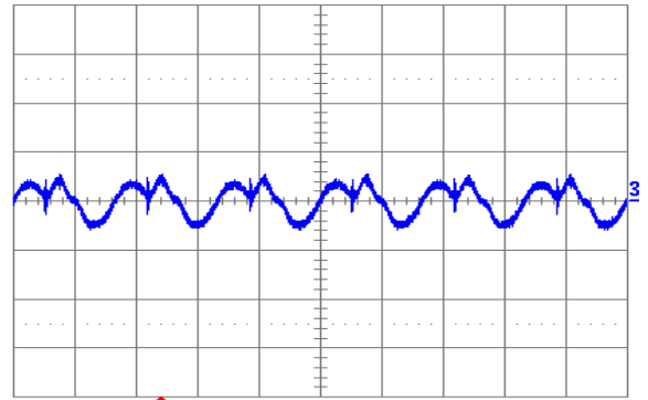
Fig. 1.5V.6: Output voltage ripple (20 mV/div.) at full rated load current into a resistive load with external capacitance 100\text{ }\mu\text{F} ceramic + 1\text{ }\mu\text{F} ceramic, and V_{in} = 12\text{ V} for V_{out} = 1.5\text{ V} . Time scale: 2 \mu\text{s} /div.
