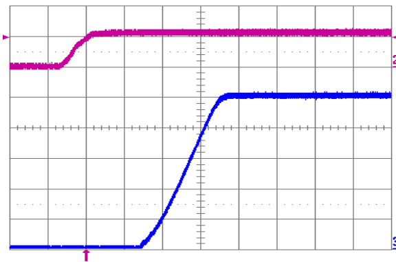
Fig. 5.0V.5: Turn-on transient for V_{out} = 5.0\text{ V} with application of V_{in} at full rated load current (resistive) and 100\text{ }\mu\text{F} external capacitance at V_{in} = 12\text{ V} . Top trace: V_{in} (10 V/div.); Bottom trace: output voltage (1 V/div.); Time scale: 2 ms/div.
