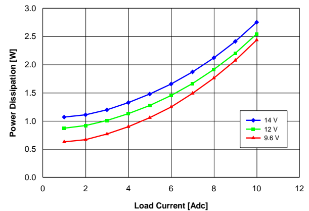
Fig. 5.0V.4: Power Loss vs. load current and input voltage for V_{out} = 5.0\text{ V} converter mounted vertically with air flowing at a rate of 200 LFM (1 m/s) and T_a = 25\text{ }^{\circ}\text{C} .
