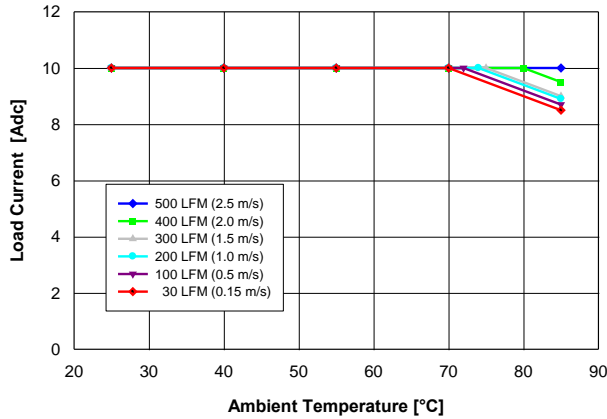
Fig. 5.0V.1: Available load current vs. ambient temperature and airflow rates for V_{out} = 5.0\text{ V} converter mounted vertically with V_{in} = 12\text{ V} , and maximum MOSFET temperature \leq 110\text{ }^{\circ}\text{C} .
