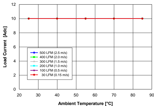
Fig. 1.5V.1: Available load current vs. ambient temperature and airflow rates for V_{out} = 1.5\text{ V} converter mounted vertically with V_{in} = 12\text{ V} , and maximum MOSFET temperature \leq 110\text{ }^\circ\text{C} .
