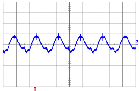
Fig. 5.0V.6: Output voltage ripple (20 mV/div.) at full rated load current into a resistive load with external capacitance 100\text{ }\mu\text{F} ceramic + 1\text{ }\mu\text{F} ceramic, and V_{in} = 12\text{ V} for V_{out} = 5.0\text{ V} . Time scale: 2 μs/div.
