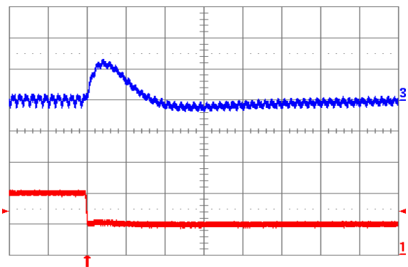
Fig. 2.5V.8: Output voltage response for V_{out} = 2.5\text{ V} to negative load current step change from 10 A to 5 A with slew rate of -5 A/ \mu\text{s} at V_{in} = 12\text{ V} . Top trace: output voltage (100 mV/div.); Bottom trace: load current (5 A/div.). C_o = 100\text{ }\mu\text{F} ceramic. Time scale: 20 \mu\text{s} /div.
