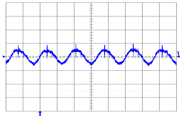
Fig. 2.0V.6: Output voltage ripple (20 mV/div.) at full rated load current into a resistive load with external capacitance 100\text{ }\mu\text{F} ceramic + 1\text{ }\mu\text{F} ceramic, and V_{in} = 12\text{ V} for V_{out} = 2.0\text{ V} . Time scale: 2 \mu\text{s} /div.
