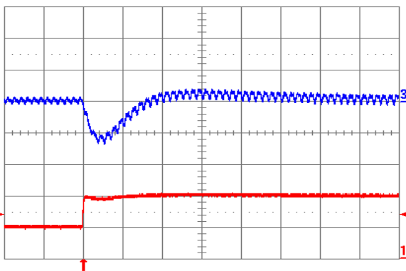
Fig. 2.5V.7: Output voltage response for V_{out} = 2.5\text{ V} to positive load current step change from 5 A to 10 A with slew rate of 5 A/ \mu\text{s} at V_{in} = 12\text{ V} . Top trace: output voltage (100 mV/div.); Bottom trace: load current (5 A/div.). C_o = 100\text{ }\mu\text{F} ceramic. Time scale: 20 \mu\text{s} /div.
