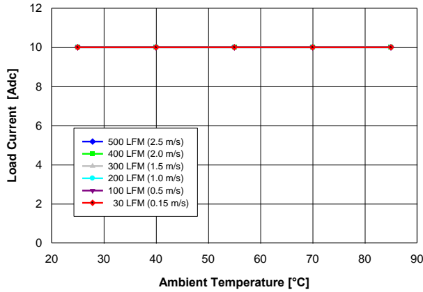
Fig. 1.2V.1: Available load current vs. ambient temperature and airflow rates for V_{out} = 1.2\text{ V} converter mounted vertically with V_{in} = 12\text{ V} , and maximum MOSFET temperature \leq 110\text{ }^{\circ}\text{C} .
