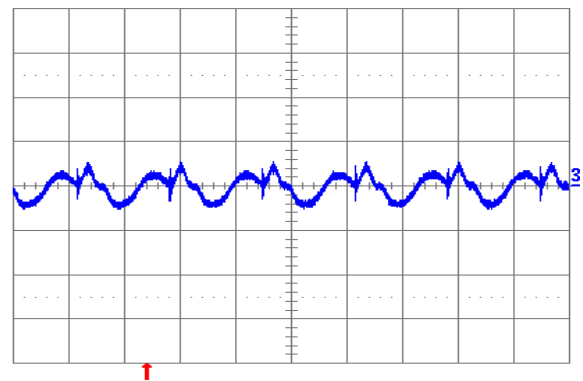
Fig. 1.2V.6: Output voltage ripple (20 mV/div.) at full rated load current into a resistive load with external capacitance 100\text{ }\mu\text{F} ceramic + 1\text{ }\mu\text{F} ceramic, and V_{in} = 12\text{ V} for V_{out} = 1.2\text{ V} . Time scale: 2\text{ }\mu\text{s}/\text{div} .
