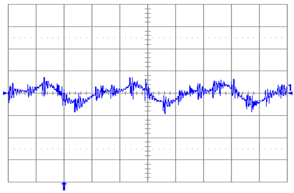
Fig. 2.5V.6: Output voltage ripple (20 mV/div.) at full rated load current into a resistive load with external capacitance 47\text{ }\mu\text{F} ceramic + 1\text{ }\mu\text{F} ceramic, and V_{in} = 5\text{ V} for V_{out} = 2.5\text{ V} . Time scale: 2 \mu\text{s} /div.
