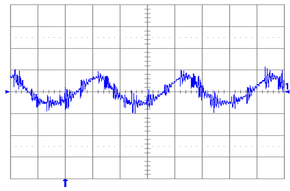
Fig. 3.3V.6: Output voltage ripple (20 mV/div.) at full rated load current into a resistive load with external capacitance 47\text{ }\mu\text{F} ceramic + 1\text{ }\mu\text{F} ceramic, and V_{in} = 5\text{ V} for V_{out} = 3.3\text{ V} . Time scale: 2 \mu\text{s} /div.
