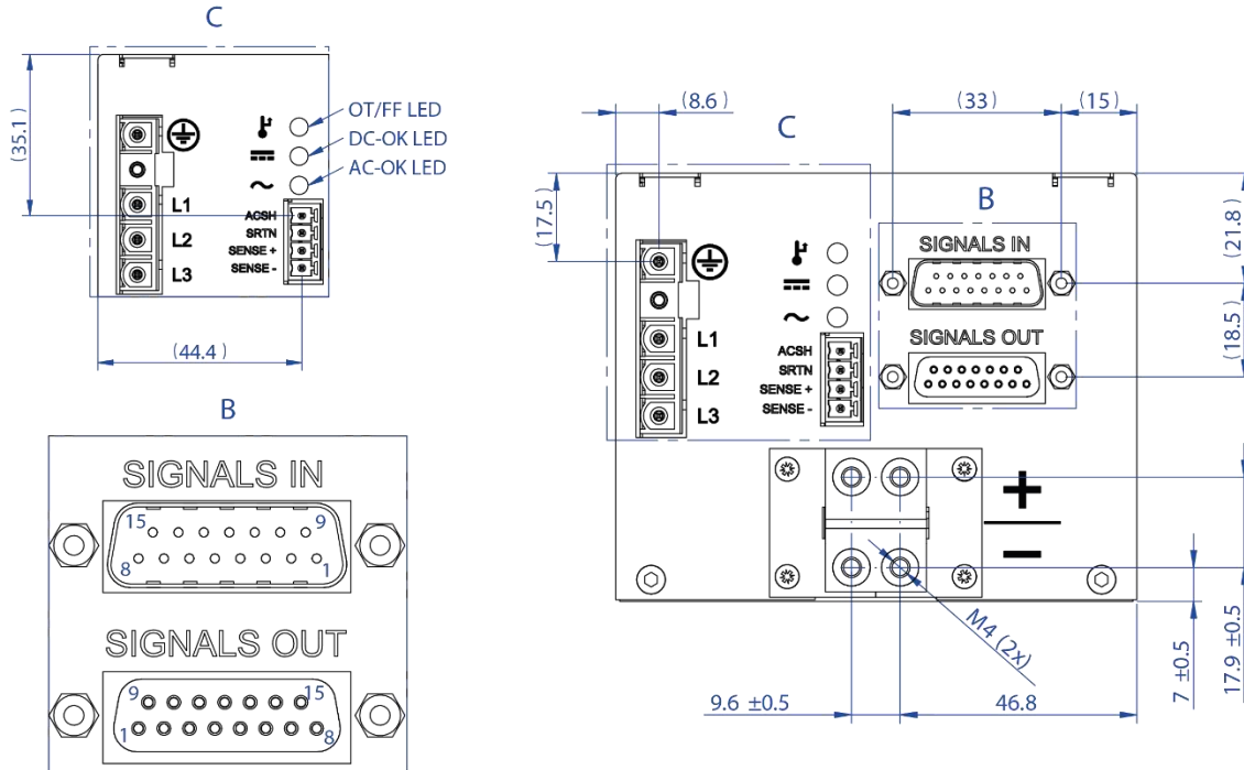
Figure 1. TCP4000- H090 - Connectors Position
