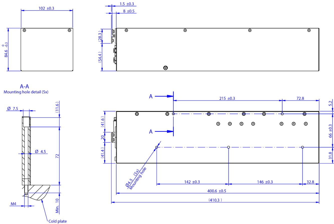
Figure 2. Mechanical Dimensions
