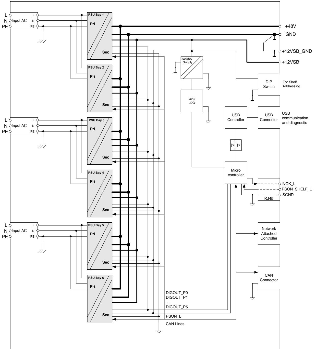
Figure 1. SPSTET4-02 Block Diagram
