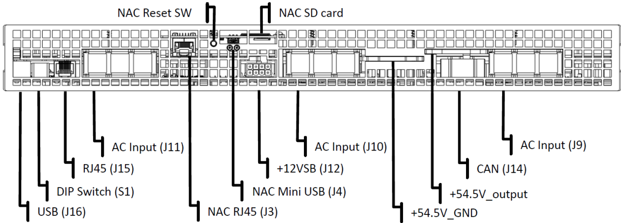
Figure 3. SPSTET4-02 Front View
