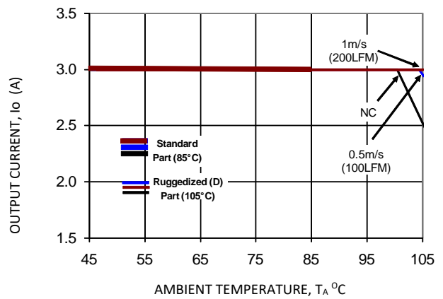
Figure 12. V_o = 5.0 V
