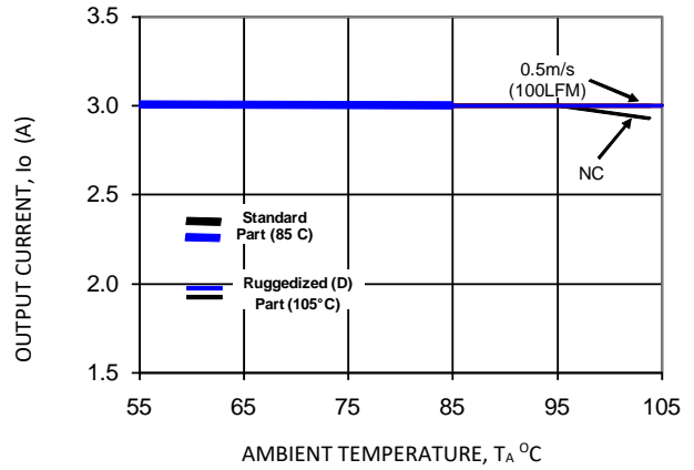
Figure 8. V_o = 1.2 V
