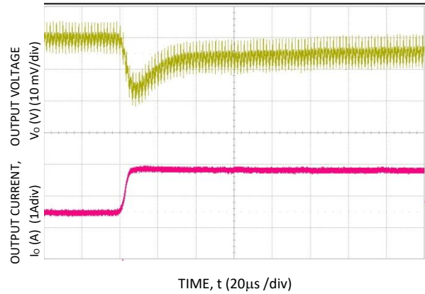
Figure 20. Transient Response to Dynamic Load Change from 50% to 100% at 12 Vin, Cout = 1x 47 \mu F + 1x 330 \mu F, CTune = 10 nF & RTune = 267 \Omega . Vo = 1.2 V
