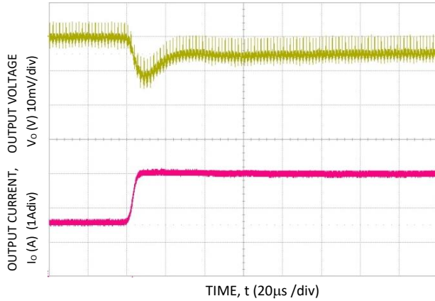
Figure 19. Transient Response to Dynamic Load Change from 50% to 100% at 12 Vin, Cout = 1x 47 \mu F + 2x 330 \mu F, CTune = 27 nF, RTune = 180 \Omega . Vo = 0.6 V
