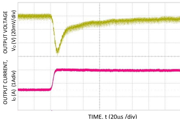
Figure 23. Transient Response to Dynamic Load Change from 50% to 100% at 12 Vin, Cout = 2x 47 \mu F, CTune = 2200 pF & RTune = 267 \Omega . Vo = 3.3 V
