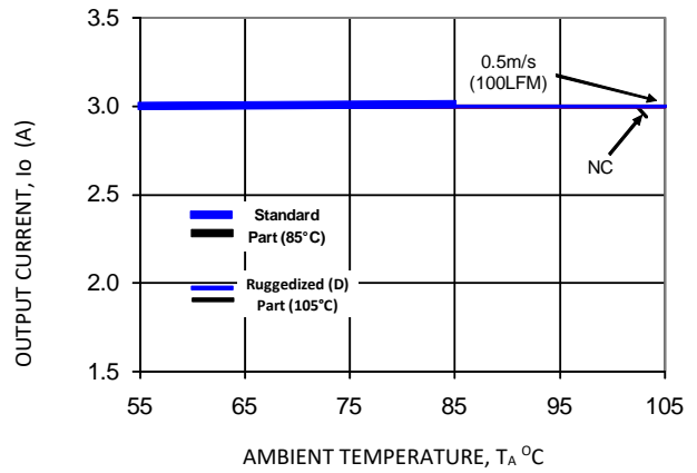
Figure 10. V_o = 2.5 V
