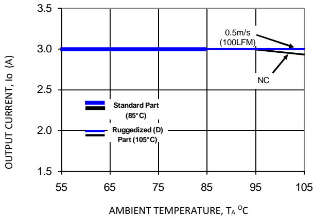
Figure 9. V_o = 1.8 V
