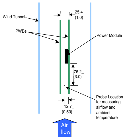
Figure 49. Thermal Test Setup
