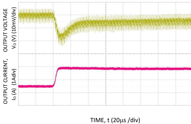
Figure 21. Transient Response to Dynamic Load Change from 50% to 100% at 12 Vin, Cout = 1x 47 \mu F + 1x 330 \mu F, CTune = 10 nF & RTune = 267 \Omega . Vo = 1.8 V
