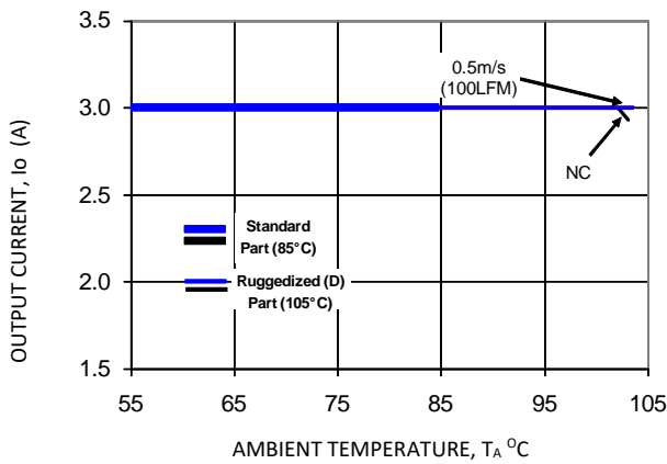
Figure 11. V_o = 3.3 V
