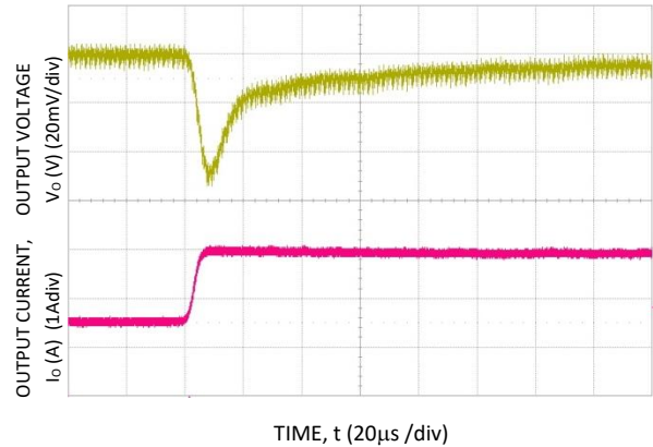
Figure 22. Transient Response to Dynamic Load Change from 50% to 100% at 12 Vin, Cout = 2x 47 \mu F, CTune = 2700 pF & RTune = 267 \Omega . Vo = 2.5 V
