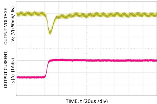
Figure 24. Transient Response to Dynamic Load Change from 50% to 100% at 12 Vin, Cout = 1x 47 \mu F, CTune = 820 pF & RTune = 267 \Omega . Vo = 5.0 V
