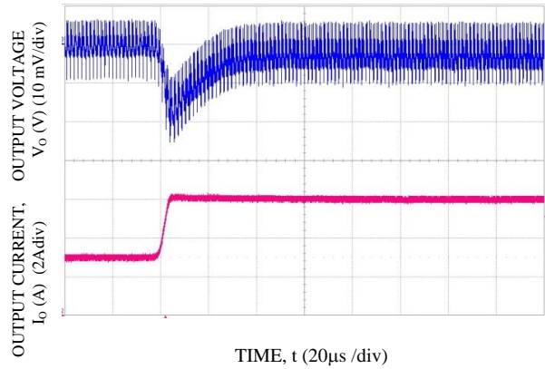
Figure 32. Transient Response to Dynamic Load Change from 50% to 100% at 12 Vin, Cout-1x47 uF+3x330 uF, CTune-12 nF & RTune-178 Ω. Vo = 1.2 V
