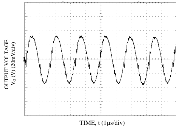
Figure 18. V_o = 5.0\text{ V} , I_o = I_{o, \text{max}} , V_{in} = 12\text{ V}
