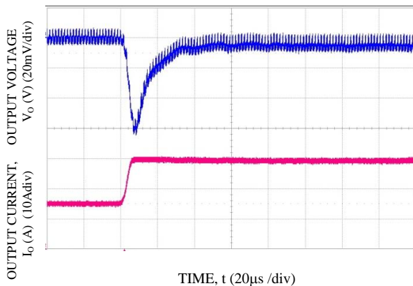
Figure 35. Transient Response to Dynamic Load Change from 50% to 100% at 12 Vin, Cout-3x47 uF, CTune-3900 pf & RTune- 178 Ω. Vo = 3.3 V
