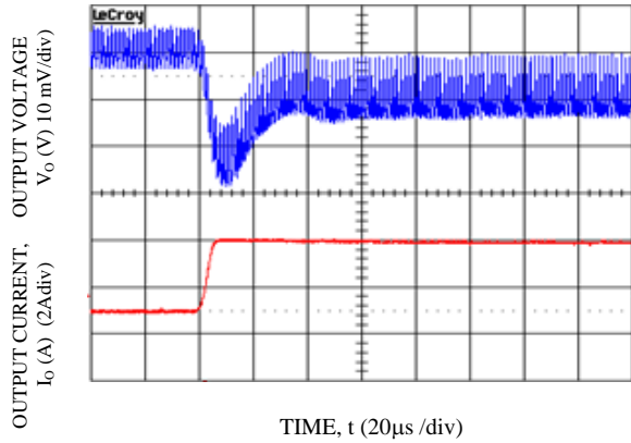
Figure 31. Transient Response to Dynamic Load Change from 50% to 100% at 8 Vin, Cout-1x47 uF+4x330 uF, CTune-33 nF, RTune-178 Ω. Vo = 0.6 V
