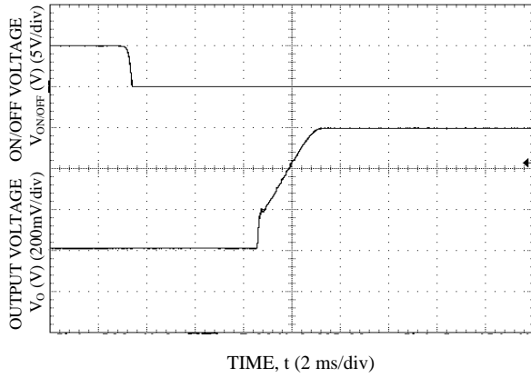
Figure 19. Start-up Using On/Off Voltage ( I_o = I_{o,max} ), V_o = 0.6 V
