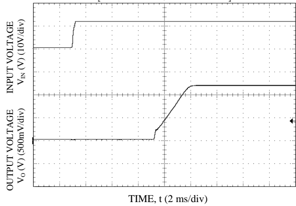
Figure 26. Start-up Using Input Voltage ( V_{IN} = 12\text{ V} , I_o = I_{o,max} ), V_o = 1.2\text{ V}
