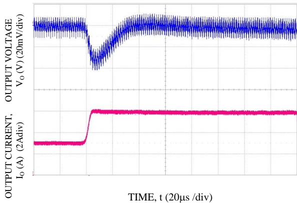
Figure 33. Transient Response to Dynamic Load Change from 50% to 100% at 12 Vin, Cout-1x47 uF+1x330 uF, CTune-4700 pF & RTune-178 Ω. Vo = 1.8 V
