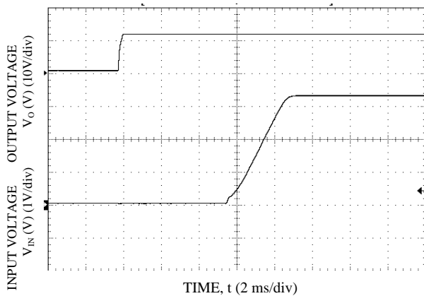
Figure 29. Start-up Using Input Voltage ( V_{IN} = 12\text{ V} , I_o = I_{o,max} ), V_o = 3.3\text{ V}
