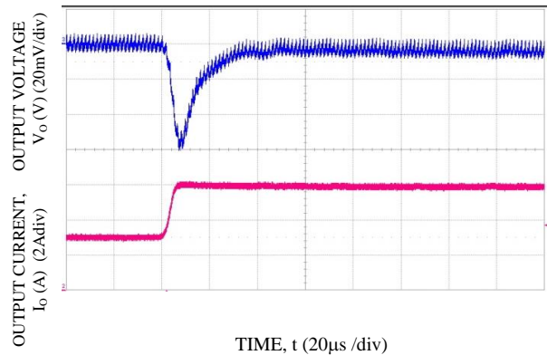
Figure 34. Transient Response to Dynamic Load Change from 50% to 100% at 12 Vin, Cout-3x47 uF, CTune-3300 pF & RTune-178 Ω. Vo = 2.5 V
