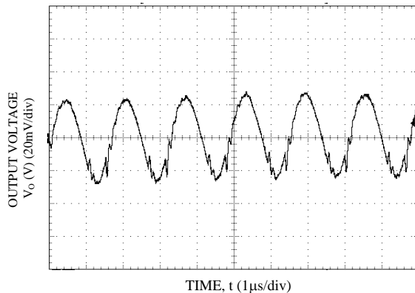
Figure 17. V_o = 3.3\text{ V} , I_o = I_{o, \text{max}} , V_{in} = 12\text{ V}
