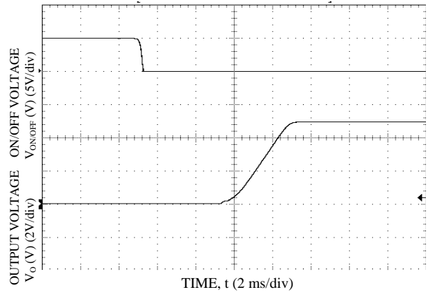
Figure 24. Start-up Using On/Off Voltage ( I_o = I_{o,max} ), V_o = 5.0 V
