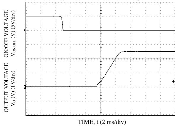
Figure 22. Start-up Using On/Off Voltage ( I_o = I_{o,max} ), V_o = 2.5 V
