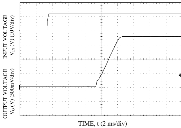
Figure 27. Start-up Using Input Voltage ( V_{IN} = 12\text{ V} , I_o = I_{o,max} ), V_o = 1.8\text{ V}
