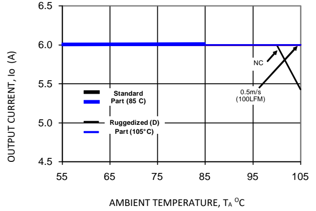
Figure 8. V_o = 1.2 V
