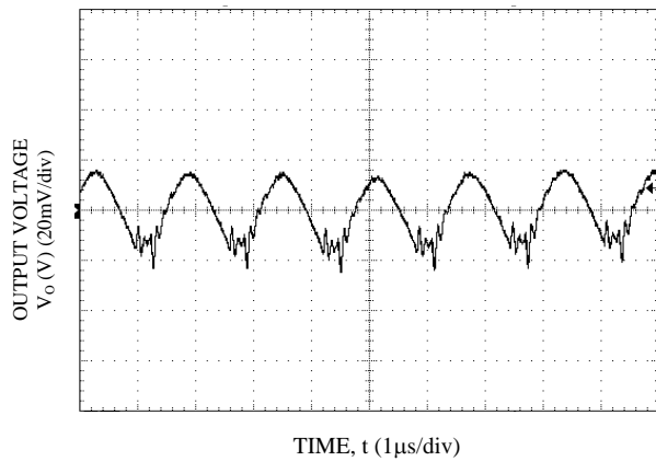
Figure 15. V_o = 1.8\text{ V} , I_o = I_{o, \text{max}} , V_{in} = 12\text{ V}
