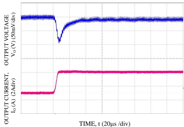
Figure 36. Transient Response to Dynamic Load Change from 50% to 100% at 12 Vin, Cout-2x47 uF, CTune-2200 pF & RTune-261 Ω. Vo = 5 V
