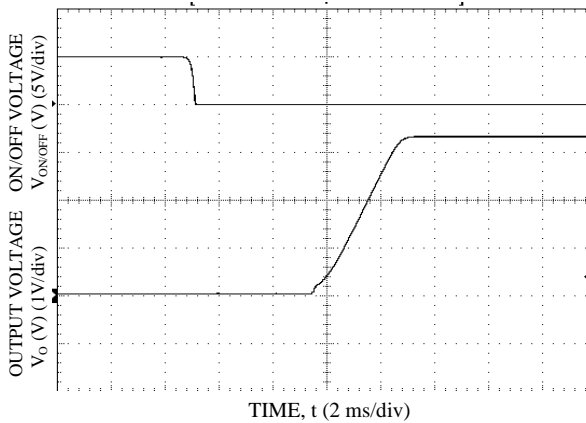
Figure 23. Start-up Using On/Off Voltage ( I_o = I_{o,max} ), V_o = 3.3 V
