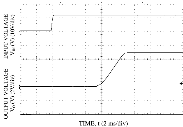
Figure 30. Start-up Using Input Voltage ( V_{IN} = 12\text{ V} , I_o = I_{o,max} ), V_o = 5.0\text{ V}
