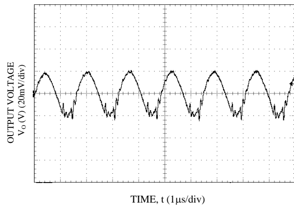
Figure 16. V_o = 2.5\text{ V} , I_o = I_{o, \text{max}} , V_{in} = 12\text{ V}
