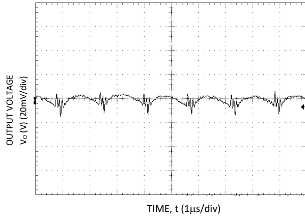
Figure 13. V_o = 0.6\text{ V} , I_o = I_{o, \text{max}} , V_{in} = 12\text{ V}
