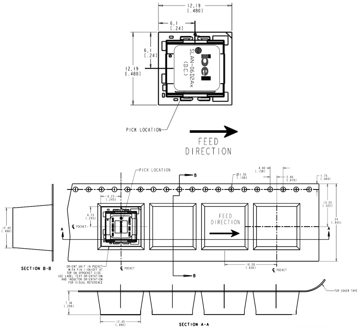
Figure 52. Packaging details
