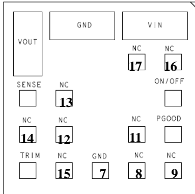
Figure 50. Pins
