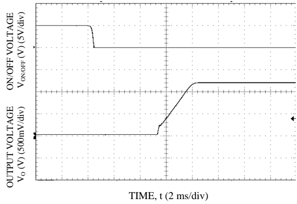
Figure 20. Start-up Using On/Off Voltage ( I_o = I_{o,max} ), V_o = 1.2 V
