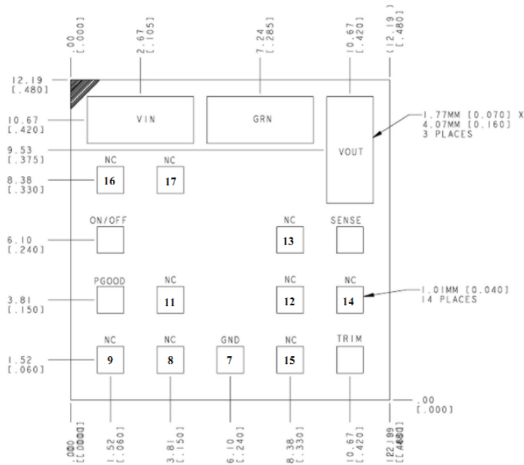
Figure 51. Recommended pad layout
