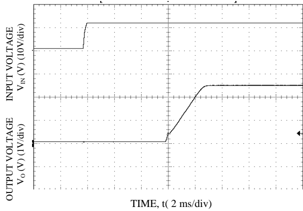
Figure 28. Start-up Using Input Voltage ( V_{IN} = 12\text{ V} , I_o = I_{o,max} ), V_o = 2.5\text{ V}
