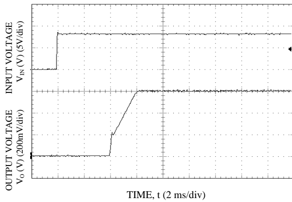
Figure 25. Start-up Using Input Voltage ( V_{IN} = 8\text{ V} , I_o = I_{o,max} ), V_o = 0.6\text{ V}
