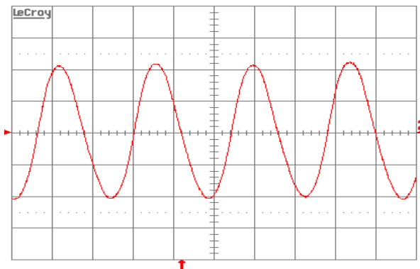
Figure 20. Input reflected ripple current, i_c (100 mA/div.), measured at input terminals at full rated load current and V_{in} = 48 V. Refer to Fig. 20 for test setup. Time scale: 1 \mu s/div.
