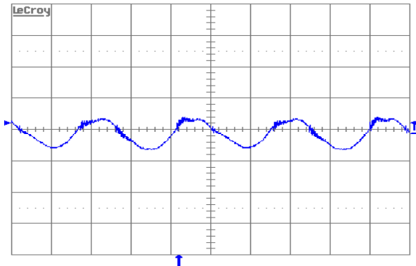
Figure 18. Output voltage ripple (50 mV/div.) at full rated load current into a resistive load with C_o = 10 \mu F tantalum + 1 \mu F ceramic and V_{in} = 48 V. Time scale:
