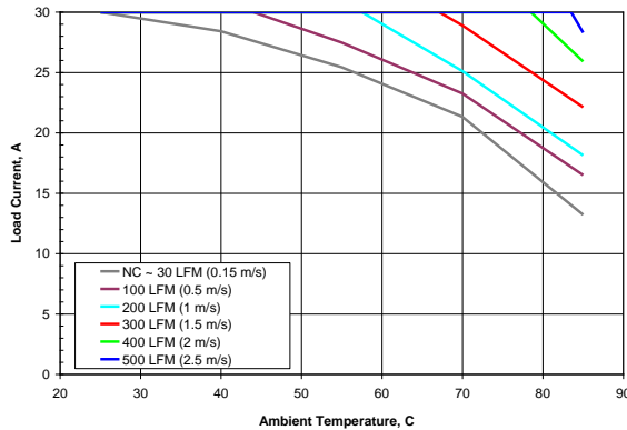
Figure 9. Available load current vs. ambient air temperature and airflow rates for converter mounted vertically with air flowing from pin 1 to pin 3, MOSFET temperature \leq 120 °C, V_{in} = 48 V. Note: NC – Natural convection
