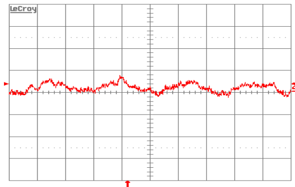
Figure 21. Input reflected ripple current, i_s (10 mA/div.), measured through 10 \mu H at the source at full rated load current and V_{in} = 48 V. Refer to Fig. 20 for test setup. Time scale: 1 \mu s/div.
