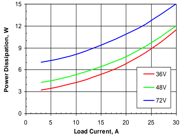
Figure 12. Power dissipation vs. load current and input voltage for converter mounted vertically with air flowing from pin 1 to pin 3 at a rate of 300 LFM (1.5 m/s) and air flowing from pin 1 to pin 3 at a rate of 200 LFM (1.0 m/s).
