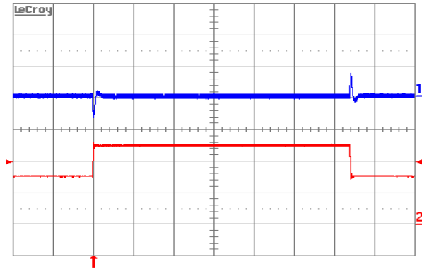
Figure 17. Output voltage response to load current step-change (15 A – 25 A – 15 A) at V_{in} = 48 V. Top trace: output voltage (200 mV/div.). Bottom trace: load current (10 A/div.). Current slew rate: 5 A/ \mu s. C_o = 470 \mu F POS + 1 \mu F ceramic. Time scale: 0.2 ms/div.
