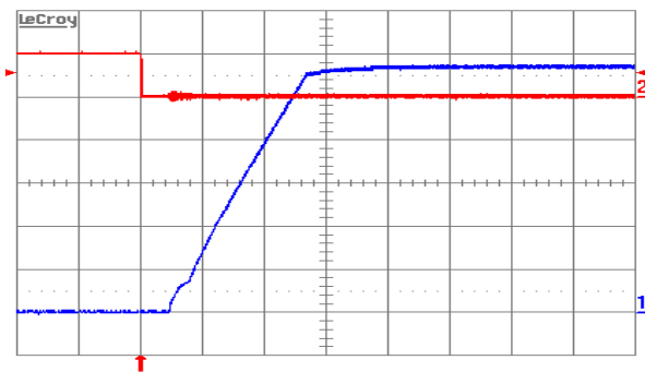
Figure 14. Turn-on transient at full rated load current (resistive) with no output capacitor at V_{in} = 48\text{ V} , triggered via ON/OFF pin. Top trace: ON/OFF signal
