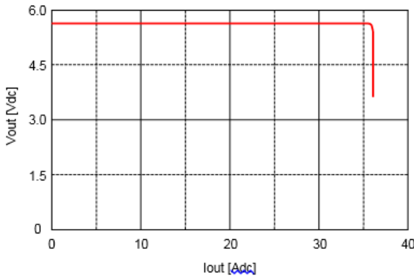
Figure 22. Output voltage vs. load current showing current limit point and converter shutdown point. Input voltage has almost no effect on current limit characteristic.
