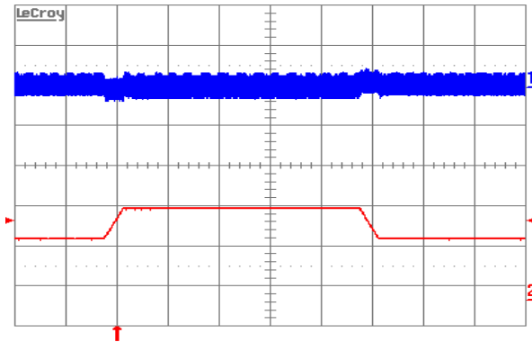
Figure 16. Output voltage response to load current step-change (15 A – 25 A – 15 A) at V_{in} = 48 V. Top trace: output voltage (100 mV/div.). Bottom trace: load current (10 A/div.). Current slew rate: 0.1 A/ \mu s. C_o = 1 \mu F ceramic. Time scale: 0.2 ms/div.
