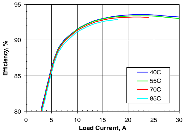
Figure 11. Efficiency vs. load current and ambient temperature for converter mounted vertically with V_{in} = 48\text{ V} and air flowing from pin 1 to pin 3 at a rate of 200 LFM (1.0 m/s).
