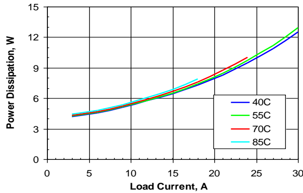
Figure 13. Power dissipation vs. load current and ambient temperature for converter mounted vertically with V_{in} = 48\text{ V} and air flowing from pin 1 to pin 3 at a rate of 200 LFM (1.0 m/s).
