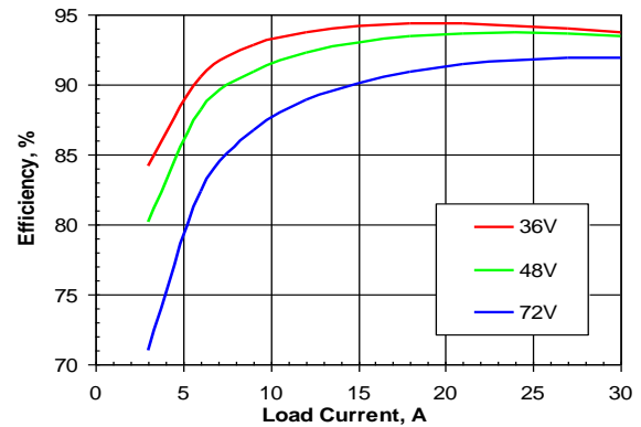
Figure 10. Efficiency vs. load current and input voltage for converter mounted vertically with air flowing from pin 1 to pin 3 at a rate of 300 LFM (1.5 m/s) and T_a = 25 °C.
