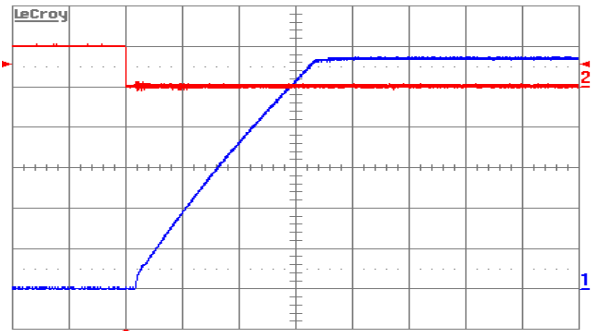
Figure 15. Turn-on transient at full rated load current (resistive) plus 10,000\ \mu\text{F} at V_{in} = 48\text{ V} , triggered via ON/OFF pin. Top trace: ON/OFF signal (5 V/div.). Bottom trace: output voltage (1 V/div.). Time scale: 5 ms/div.
