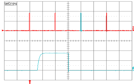
Figure 23. Load current (top trace, 20 A/div., 100 ms/div.) into a 10 mΩ short circuit during restart, at Vin = 48 V. Bottom trace (20 A/div., 2 ms/div.) is an expansion of the on-time portion of the top trace.
