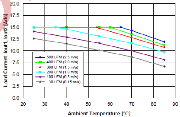
Figure 10. Available balanced load current ( I_{out1} = I_{out2} ) vs. ambient temperature and airflow rates for converter mounted with B height pins horizontally with V_{in} = 48 V, air flowing from pin 3 to pin 1 and maximum FET temperature \leq 120^{\circ}\text{C} .
