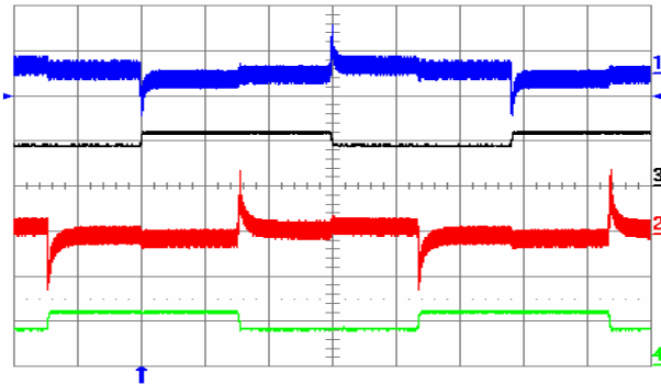
Figure 23. Output voltage response to both Iout1 and Iout2 (out of phase) load current step-change of 3.75 A (50%-75%-50%) at Vin = 48 V. Ch1 = Vout1 (50 mV/div), Ch2 = Vout2 (50 mV/div), Ch3 = Iout1 (10 A/div.), Ch4 = Iout2 (10 A/div.). Current slew rate: 0.1 A/μs, Co = 10 μF tantalum + 1 μF ceramic. Time scale: 1 ms/div.
