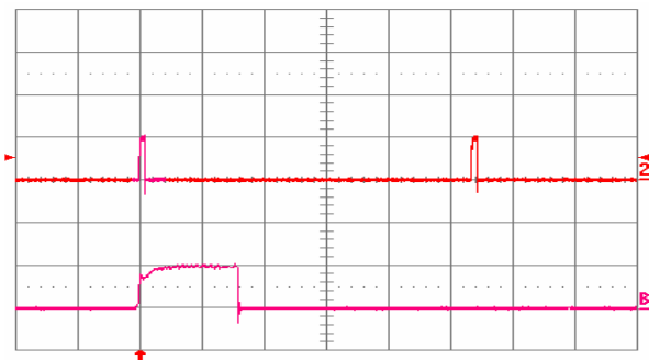
Figure 28. Load current Iout2 into a 10 mΩ short circuit on Vout2 during restart, with Vout1 open (no load), at Vin = 48 V. Ch2 = Iout2 (20 A/div, 20 ms/div). ChB = Iout2 (20 A/div, 1 ms/div) is an expansion of the on-time portion of Iout2.
