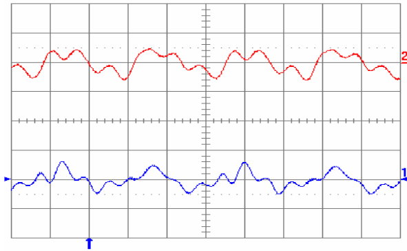
Figure 29. Output voltage ripple at full rated load current into a resistive load on both outputs with C_o = 1\mu F (ceramic) and V_{in} = 48 V . Ch2 = Vout2, Ch1 = Vout1 (both 20 mV/div). Time scale: 1 \mu s /div.
