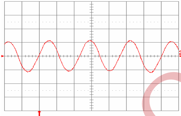
Figure 31. Input reflected ripple current, i_c (100 mA/div), measured at input terminals at full rated load current on both outputs and V_{in} = 48 V . Refer to Fig. 30 for test setup. Time scale: 1 \mu s /div.
