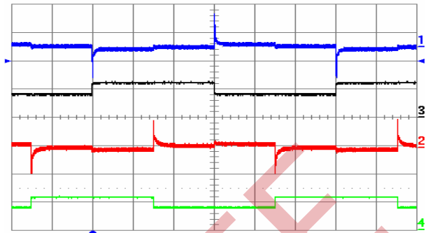
Figure 24. Output voltage response to both Iout1 and Iout2 (out of phase) load current step-change of 3.75 A (50%-75%-50%) at Vin = 48 V. Ch1 = Vout1 (100 mV/div), Ch2 = Vout2 (100 mV/div), Ch3 = Iout1 (10 A/div.), Ch4 = Iout2 (10 A/div.). Current slew rate: 0.1 A/μs, Co = 10 μF tantalum + 1 μF ceramic. Time scale: 1 ms/div.
