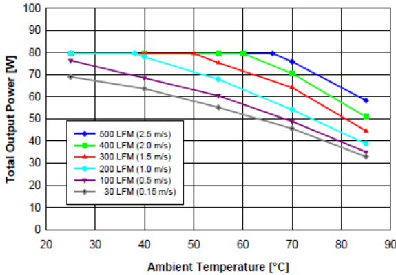
Figure 7. Available output power for balanced load current ( I_{out1} = I_{out2} ) vs. ambient air temperature and airflow rates for converter with B height pins mounted vertically with V_{in} = 48 V, air flowing from pin 3 to pin 1 and maximum FET temperature \leq 120^{\circ}\text{C} .
