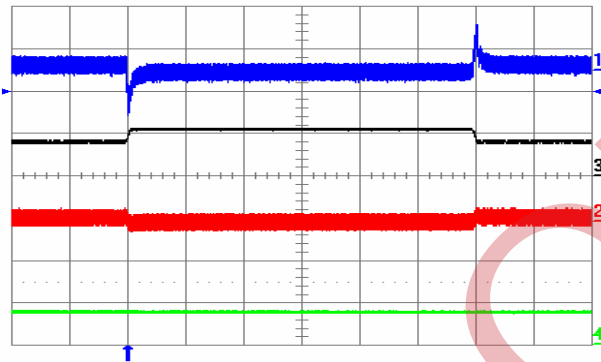
Figure 19. Output voltage response to Iout1 load current step-change of 3.75 A (50%-75%-50%) at Iout2 = 7.5 A and V_{in} = 48\text{ V} . Ch1 = Vout1 (50 mV/div), Ch2 = Vout2 (50 mV/div), Ch3 = Iout1 (10 A/div.), Ch4 = Iout2 (10 A/div.). Current slew rate: 0.1 A/ \mu\text{s} , C_o = 10\text{ }\mu\text{F} tantalum + 1 \mu\text{F} ceramic. Time scale: 0,5 ms/div.
