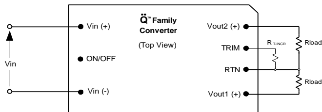
Figure 2. Configuration for increasing output voltage.
