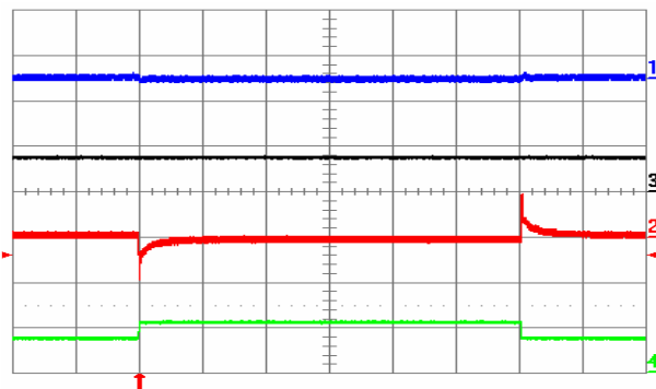
Figure 22. Output voltage response to Iout2 load current step-change of 3.75 A (50%-75%-50%) at Iout1 = 7.5 A and V_{in} = 48\text{ V} . Ch1 = Vout1 (100 mV/div), Ch2 = Vout2 (100 mV/div), Ch3 = Iout1 (10 A/div.), Ch4 = Iout2 (10 A/div.). Current slew rate: 5 A/ \mu\text{s} , C_o = 300\text{ }\mu\text{F} tantalum + 1 \mu\text{F} ceramic. Time scale: 0,5 ms/div.
