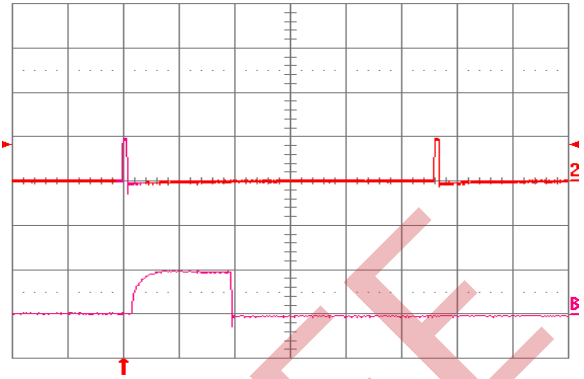
Figure 30. Load current I_{out2} into a 10\text{ m}\Omega short circuit on V_{out2} during restart, with V_{out1} open (no load), at V_{in} = 48\text{ V} . Ch2 = I_{out2} (20 A/div, 20 ms/div). ChB = I_{out2} (20 A/div, 1 ms/div) is an expansion of the on-time portion of I_{out2} .
