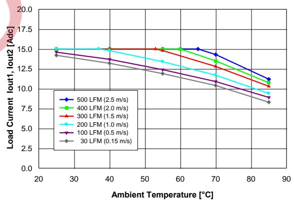
Figure 10. Available balanced load current (Iout1 = Iout2) vs. ambient air temperature and airflow rates for converter mounted horizontally with Vin = 48 V, air flowing from pin 3 to pin 4 and maximum FET temperature ≤ 120 °C.
