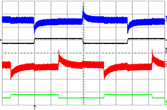
Figure 27. Output voltage response to both Iout1 and Iout2 (out of phase) load current step-change of 3.75 A (Iout1) and 2.5 A (Iout2) (50%-75%-50%) at Vin = 48 V. Ch1 = Vout1 (50 mV/div), Ch2 = Vout2 (50 mV/div), Ch3 = Iout1 (10 A/div.), Ch4 = Iout2 (10 A/div.). Current slew rate: 0.1 A/μs, Co = 10 μF tantalum + 1 μF ceramic. Time scale: 1.0 ms/div.
