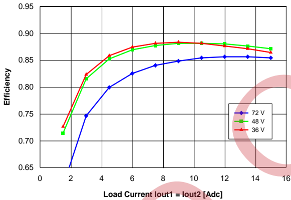
Figure 19. Efficiency vs. balanced load current (Iout1 = Iout2) and input voltage for converter mounted vertically with air flowing from pin 3 to pin 1 at a rate of 300 LFM (1.5 m/s) and Ta = 25 °C.
