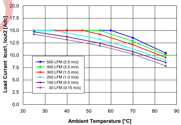
Figure 10. Available balanced load current ( I_{out1} = I_{out2} ) vs. ambient temperature and airflow rates for converter mounted horizontally with V_{in} = 48 V, air flowing from pin 3 to pin 4 and maximum FET temperature \leq 120 °C.
