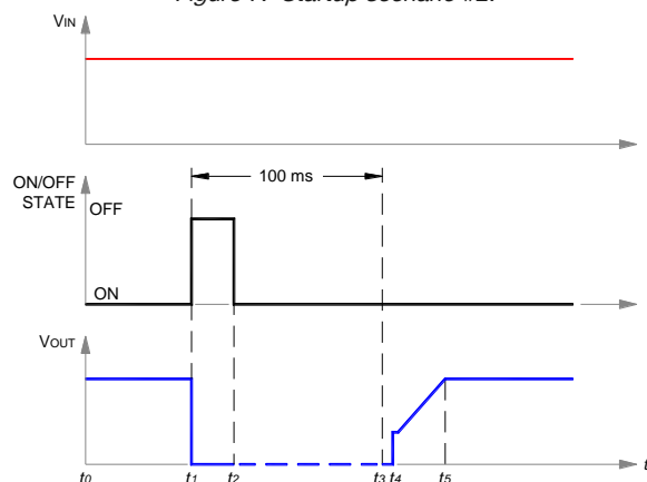
Figure 8. Startup scenario #3.
