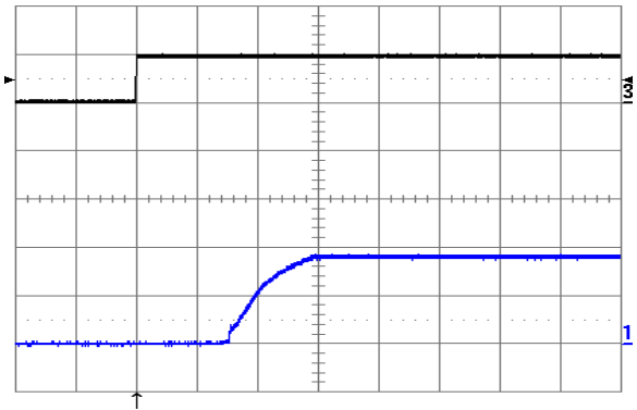
Figure 18. Turn-on transient at full rated load current (resistive) plus 10,000\text{ }\mu\text{F} at V_{in} = 48\text{ V} , triggered via ON/OFF pin. Top trace: ON/OFF signal (5 V/div.). Bottom trace: output voltage (1 V/div.). Time scale: 1 ms/div.
