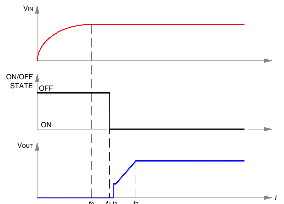
Figure 7. Startup scenario #2.
