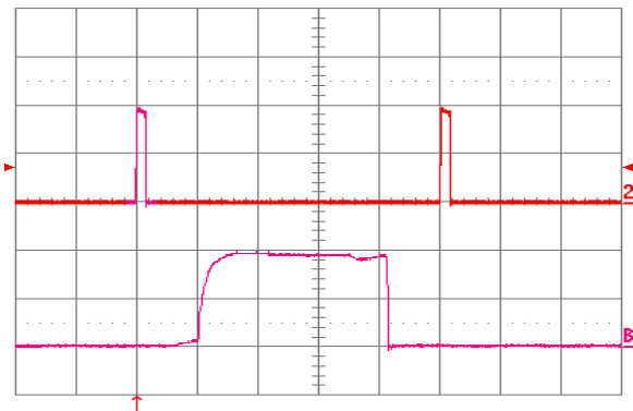
Figure 26. Load current (top trace, 20 A/div, 20 ms/div) into a 10 mΩ short circuit during restart, at V_{in} = 48 V. Bottom trace (20 A/div, 1 ms/div) is an expansion of the on-time portion of the top trace..
