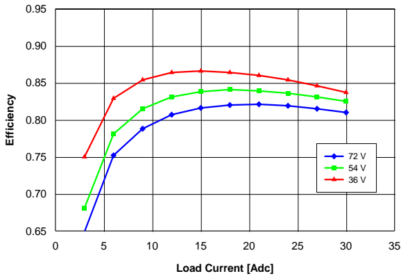
Figure 15. Efficiency vs. load current and input voltage for converter mounted horizontally with air flowing from pin 3 to pin 4 at a rate of 300 LFM (1.5 m/s) and T_a = 25\text{ }^\circ\text{C} .
