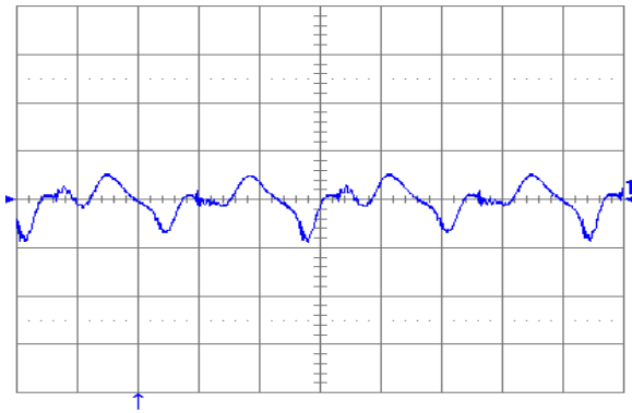
Figure 21. Output voltage ripple (20 mV/div.) at full rated load current into a resistive load with C_o = 10 \mu F tantalum + 1 \mu F ceramic and V_{in} = 48 V. Time scale: 1 \mu /div.
