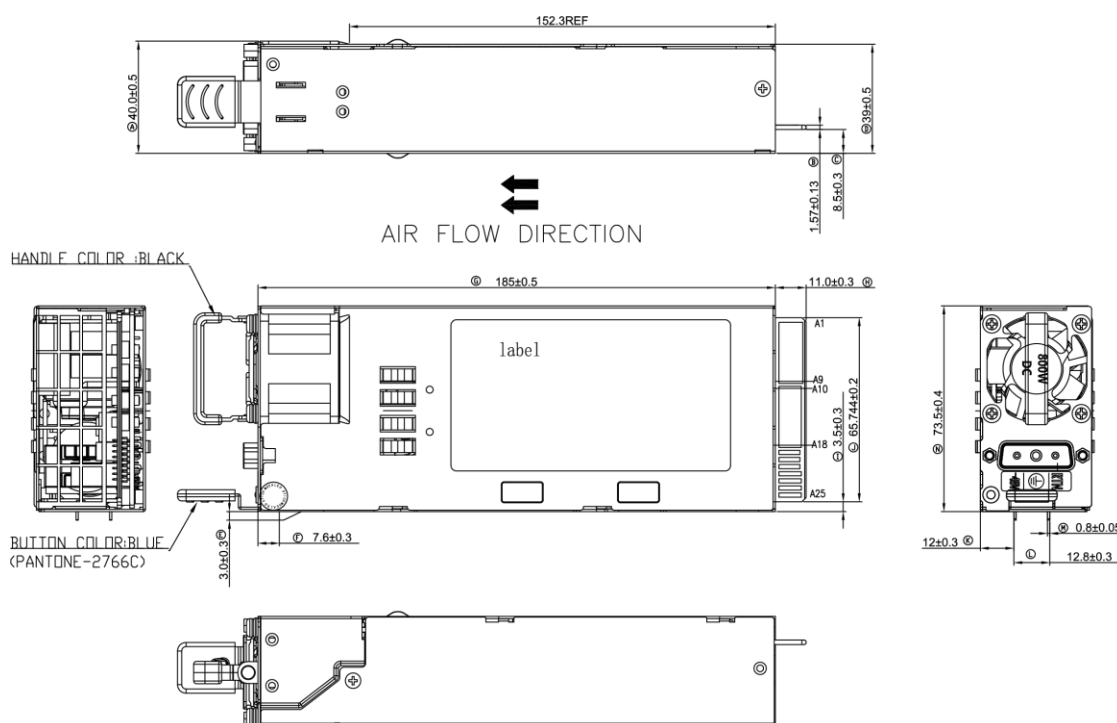
Figure 5. Mechanical Drawing
