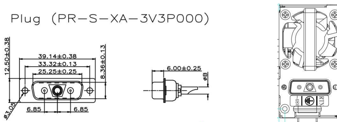
Figure 6. DC inlet connector PR-S-XA-3V3P000
