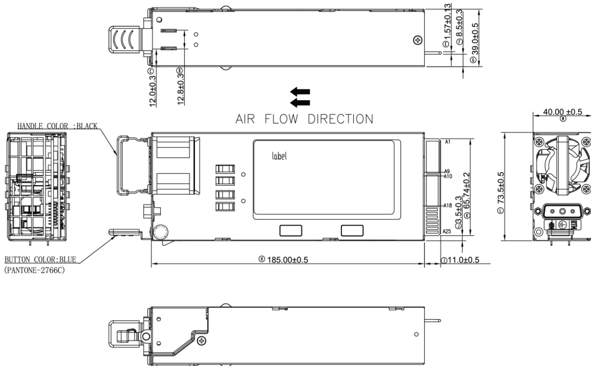
Figure 5. Mechanical Drawing
