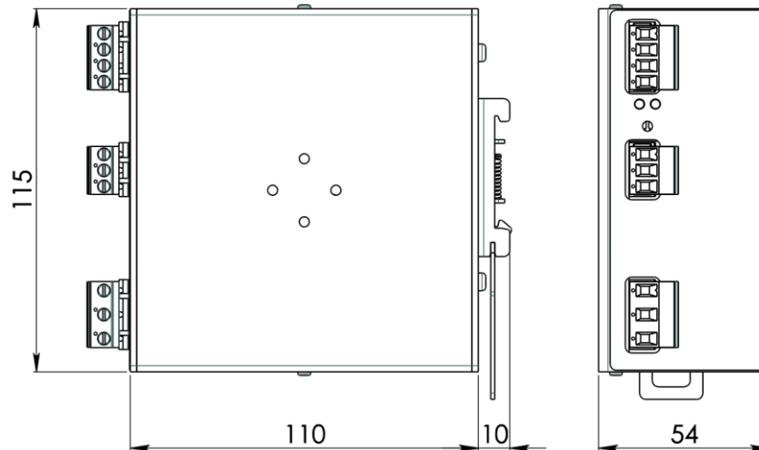
Figure 1. Mechanical Drawing
