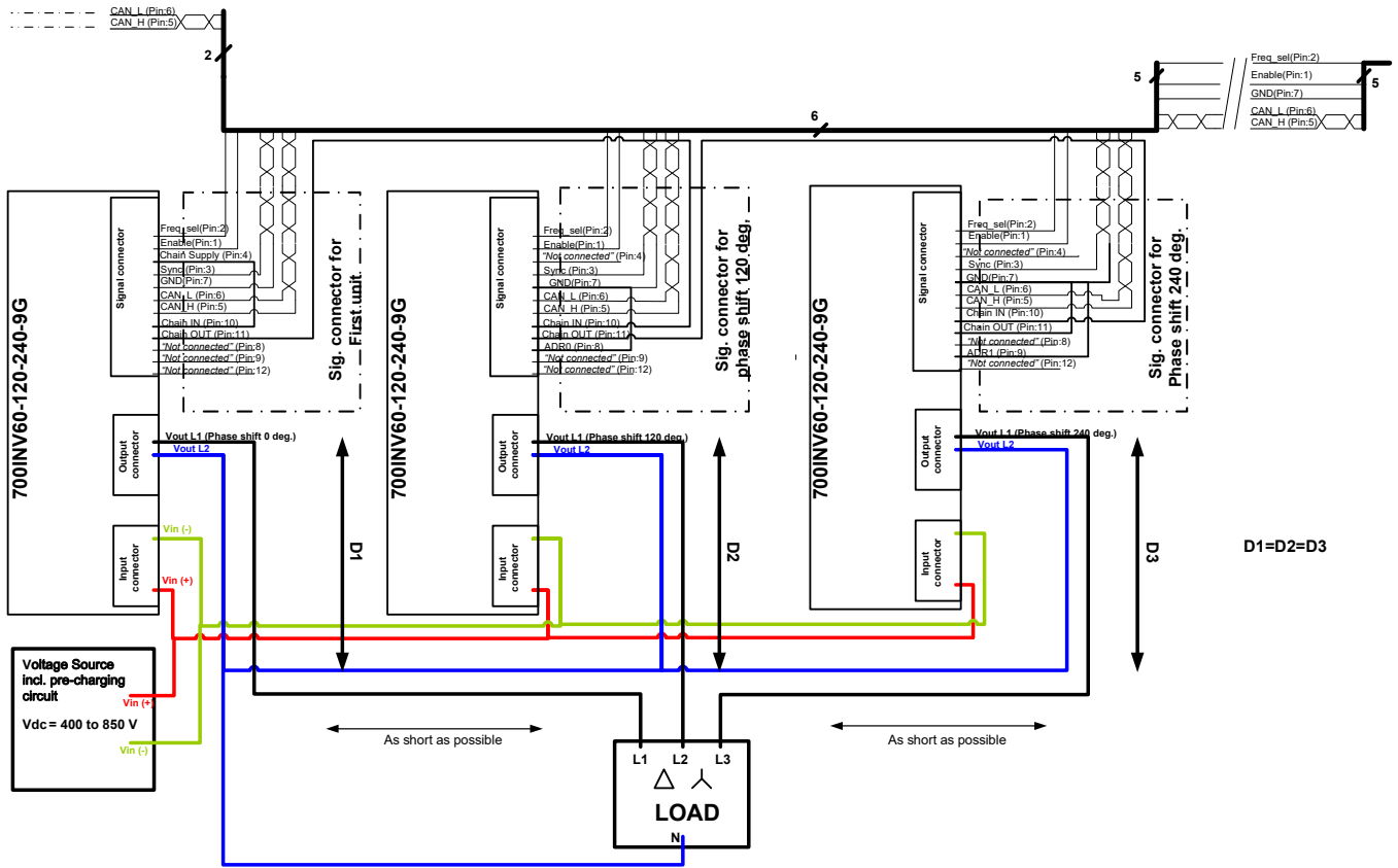
Figure 3. Wiring setup for 3-phase operation 700INV60-120-240-9G
