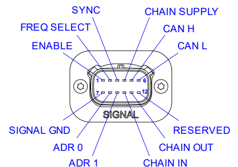
Signal Connector
