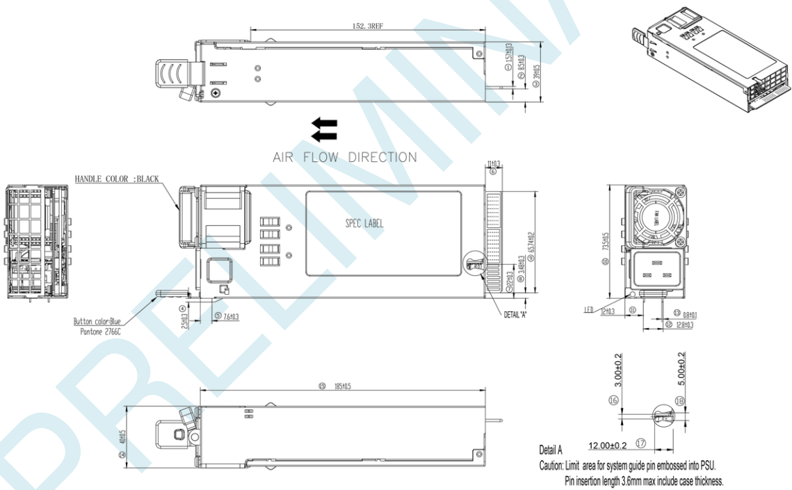
Figure 13. Mechanical Drawing
