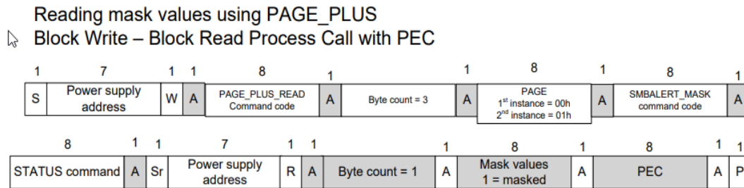
Figure 3. PAGE_PLUS_READ command.
