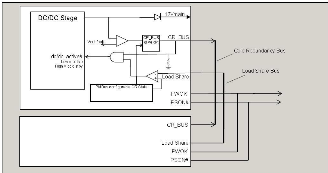
Figure 10. Cold Redundancy 1+1 Functional Block Diagram
