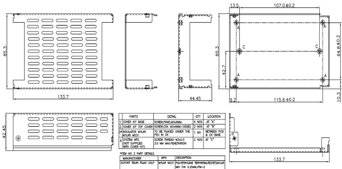
WLT200 & WLT300. MECHANICAL OUTLINE DIMENSIONS.
