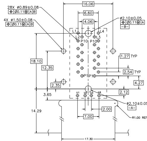
SUGGESTED CUSTOMER BOARD LAYOUT
