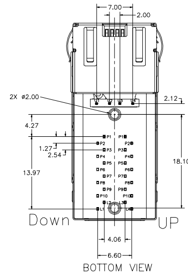
BOTTOM VIEW
