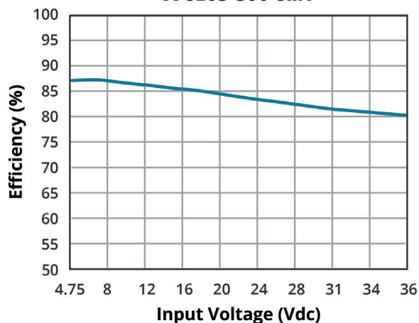
EFFICIENCY VS INPUT VOLTAGE (full load) V78E03-500-SMT
