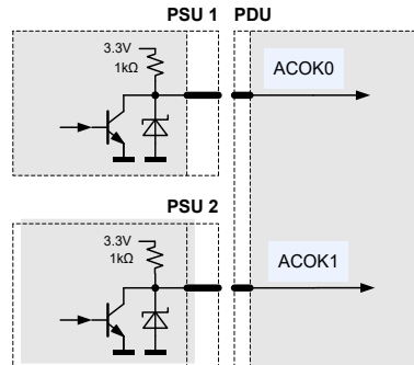
Figure 28. ACOK Connection
