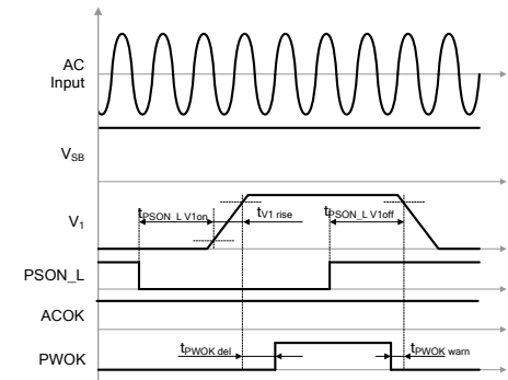
Figure 34. PSON_L Turn-on/off Timing
