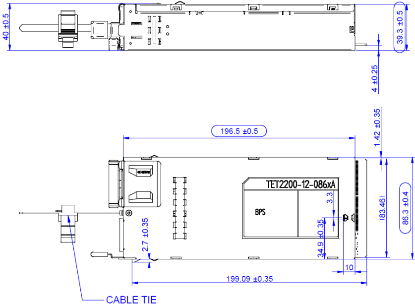
Figure 39. Mechanical Drawing - Side / Top View
