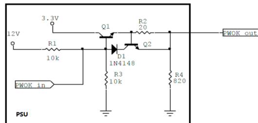
Figure 27. PWOK circuit in PSU
