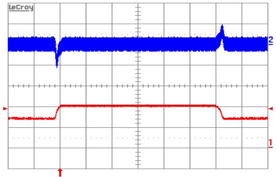
Figure 8. Output voltage response to load current step-change (6.5 A–9.75 A–6.5 A) at V_{\text{in}} = 48\text{ V} . Top trace: output voltage (100 mV/div.). Bottom trace: load current (5 A/div.). Current slew rate: 0.1 A/ \mu\text{s} . C_o = 1\mu\text{F} ceramic + 10 \mu\text{F} tantalum. Time scale: 0.2 ms/div.
