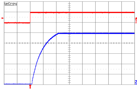
Figure 7. Turn-on transient at full rated load current (resistive) plus 10,000 \mu\text{F} at V_{\text{in}} = 48\text{ V} , triggered via ON/OFF pin. Top trace: ON/OFF signal (5 V/div.). Bottom trace: Output voltage (1 V/div.). Time scale: 5 ms/div.
