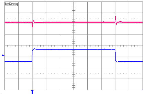
Figure 9. Output voltage response to load current step-change (25 A - 37.5 A - 25 A) at V_{in} = 48\text{ V} . Top trace: output voltage (100 mV/div.). Bottom trace: load current (10 A/div.). Current slew rate: 2.5\text{ A}/\mu\text{s} . C_o = 470\text{ }\mu\text{F POS} + 1\text{ }\mu\text{F} ceramic. Time scale: 0.2 ms/div.
