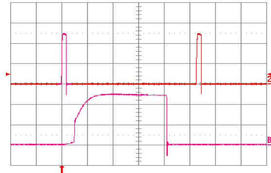
Fig. 1.8V.15: Load current (top trace, 20 A/div, 20 ms/div) into a 10 mΩ short circuit during restart, at Vin = 48 V. Bottom trace (20 A/div, 1 ms/div) is an expansion of the on-time portion of the top trace
