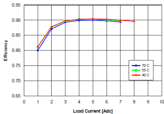
Figure 16. Efficiency vs. load current and ambient temperature for converter mounted horizontally with V_{in} = 54\text{ V} and air flowing from pin 3 to pin 4 at a rate of 200 LFM (1.0 m/s).
