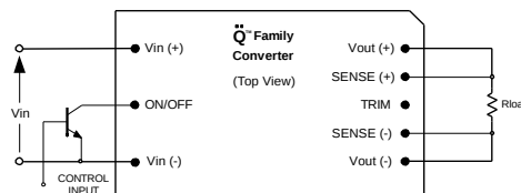
Figure 1. Circuit configuration for ON/OFF function.
