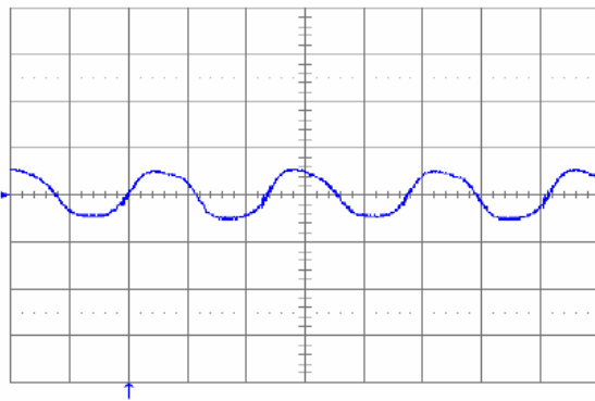
Figure 21. Output voltage ripple (50 mV/div.) at full rated load current into a resistive load with C_o = 10 \mu F tantalum + 1 \mu F ceramic and V_{in} = 48 V. Time scale: 1 \mu s/div.
