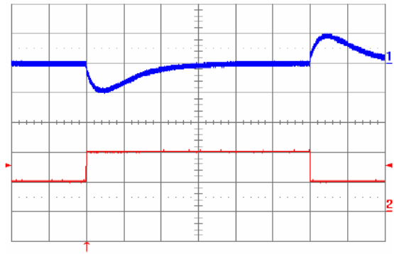
Figure 20. Output voltage response to load current step-change (2 A – 4 A – 2 A) at V_{in} = 48 V. Top trace: output voltage (200 mV/div). Bottom trace: load current (2 A/div). Current slew rate: 5 A/ \mu s. C_o = 450 \mu F tantalum + 1 \mu F ceramic. Time scale: 0.5 ms/d
