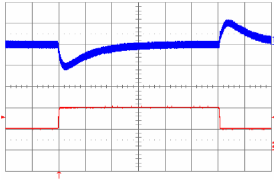
Figure 19. Output voltage response to load current step-change (2 A – 4 A – 2 A) at V_{in} = 48 V. Top trace: output voltage (200 mV/div). Bottom trace: load current (2 A/div). Current slew rate: 0.1 A/ \mu s. C_o = 1 \mu F ceramic. Time scale: 0.5 ms/div.
