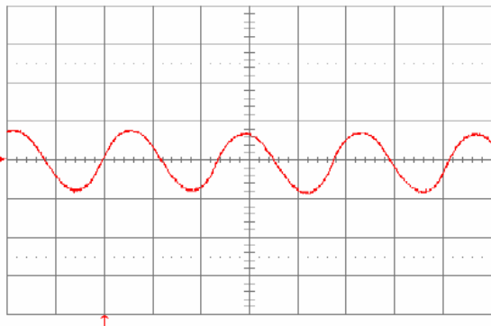
Figure 23. Input reflected ripple current, i_c (100 mA/div), measured at input terminals at full rated load current and V_{in} = 48 V. Refer to Fig. 22 for test setup. Time scale: 1 \mu s/div.
