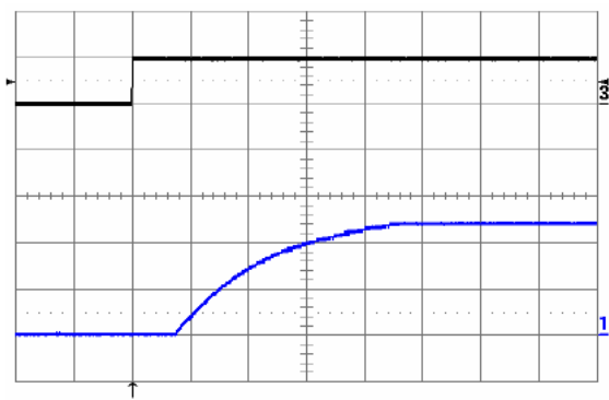
Figure 18. Turn-on transient at full rated load current (resistive) plus 2,200 \mu\text{F} at V_{in} = 48\text{ V} , triggered via ON/OFF pin. Top trace: ON/OFF signal (5 V/div.). Bottom trace: output voltage (5 V/div.). Time scale: 2 ms/div.
