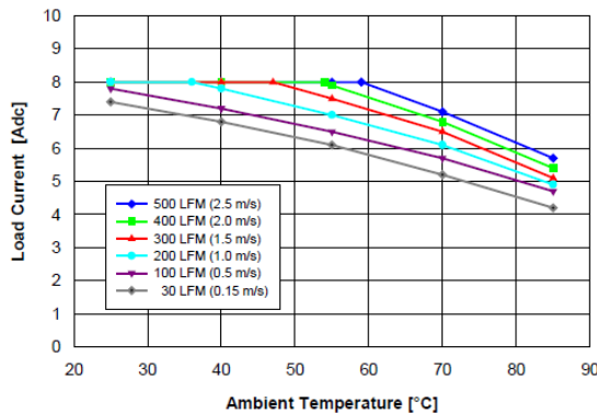
Figure 11. Available load current vs. ambient temperature and airflow rates for converter mounted horizontally with V_{in} = 54 V, air flowing from pin 3 to pin 4 and maximum FET temperature \leq 120 °C.
