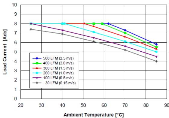
Figure 9. Available load current vs. ambient air temperature and airflow rates for converter mounted vertically with V_{in} = 54 V, air flowing from pin 3 to pin 1 and maximum FET temperature \leq 120 °C.
