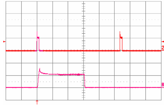
Figure 26. Load current (top trace, 10 A/div, 20 ms/div) into a 10 mΩ short circuit during restart, at V_{in} = 48 V. Bottom trace (10 A/div, 1 ms/div) is an expansion of the on-time portion of the top trace...
