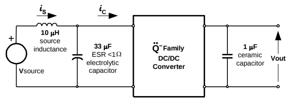
Figure 22. Test Set-up for measuring input reflected ripple currents, i_c and i_s .
