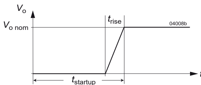
Fig. 4 Converter start-up and rise time
