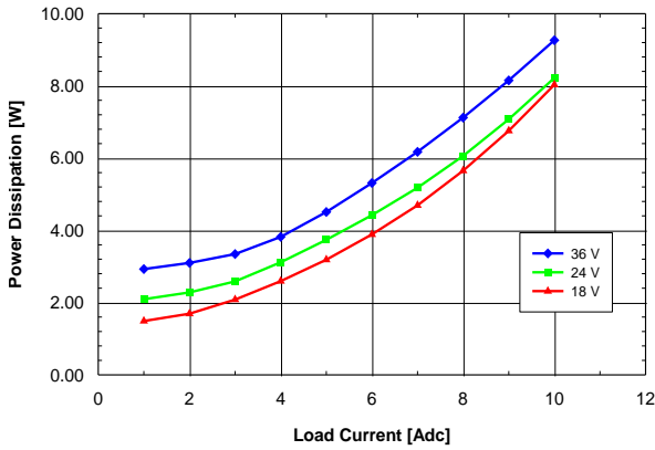
Fig. 5.0V.7: Power dissipation vs. load current and input voltage for ASQ24T/S10050 converter mounted vertically with air flowing from pin 3 to pin 1 at a rate of 300 LFM (1.5 m/s) and T_a = 25^\circ\text{C} .
