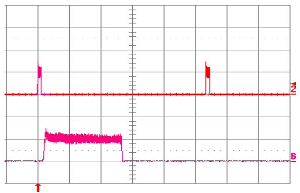
Fig. 12V.18: Load current (top trace, 5 A/div., 20 ms/div.) into a 10 \text{m}\Omega short circuit during restart, at V_{in} = 24\text{V} . Bottom trace (5 A/div., 1 ms/div.) is an expansion of the on-time portion of the top trace.
