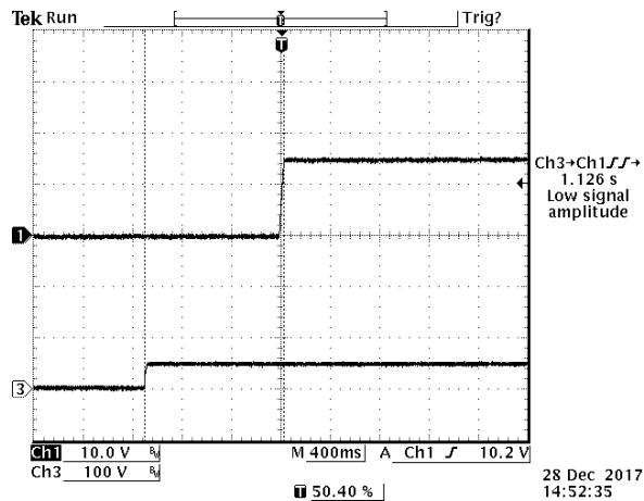
Figure 28. Startup from V_{in}
