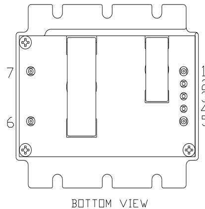
Figure 57. 0RQB-50Y15E/F Pins
