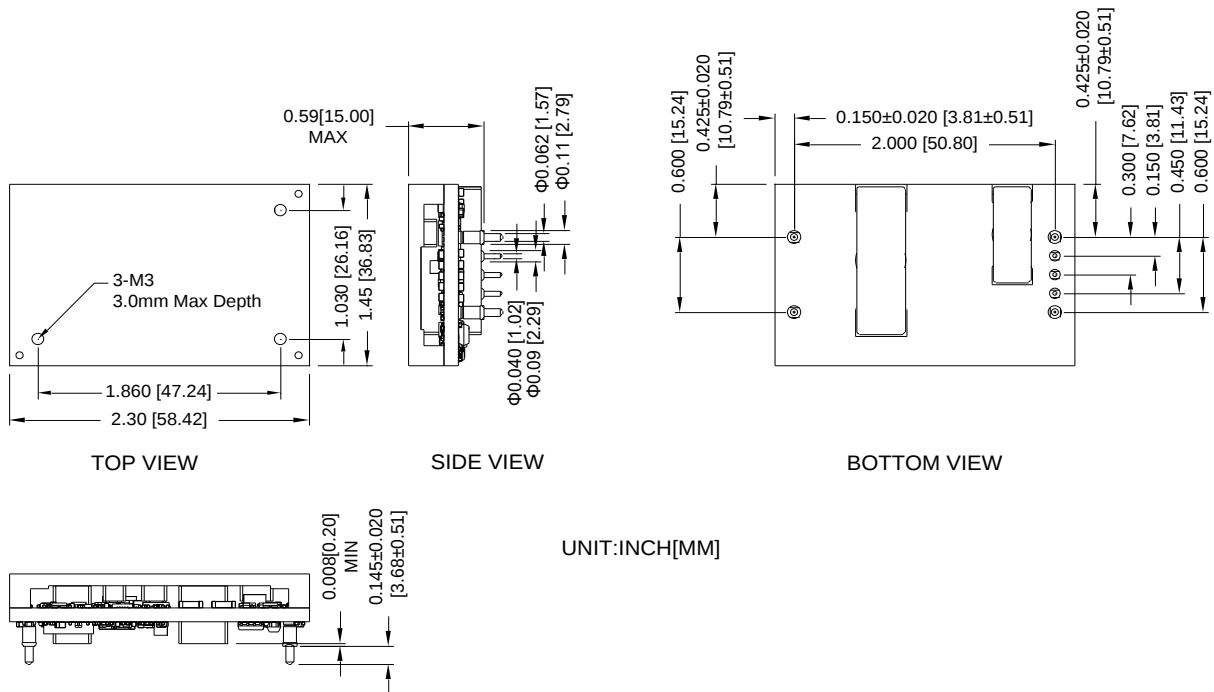
Figure 52. 0RQB-50Y15L/0 Outline
