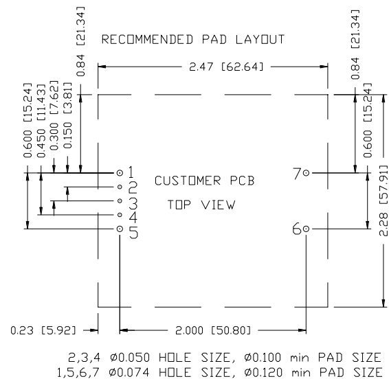
Figure 59. 0RQB-50Y15E/F Recommended pad layout-2
