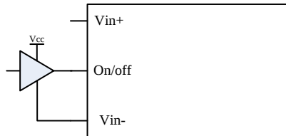
Figure 4. Control with logic circuit
