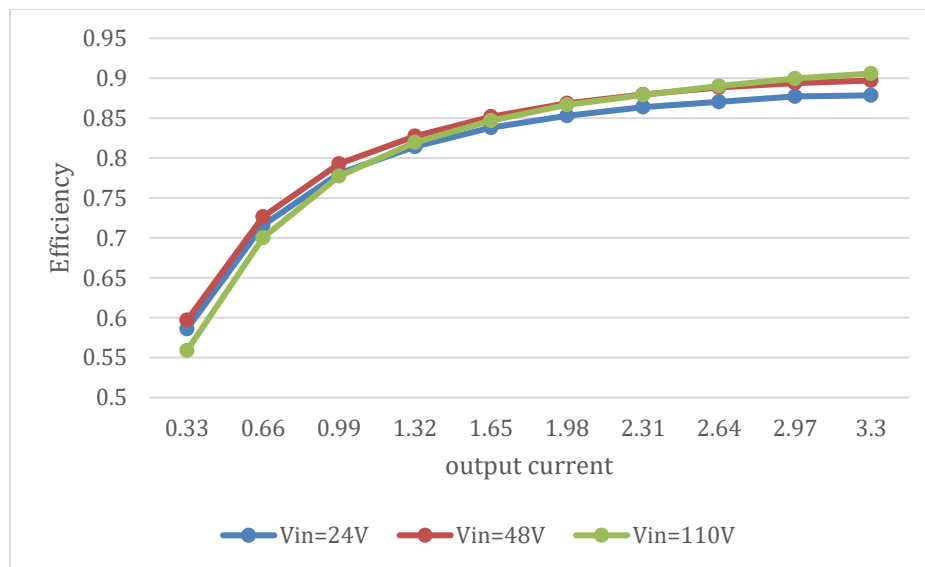
Figure 1. Efficiency data
