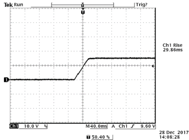
Figure 24. V_{in}=48V , I_o=3.3A , V_o=15V with C_{ext}=1200\mu F
