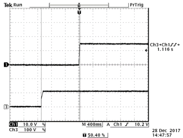
Figure 27. Startup from
