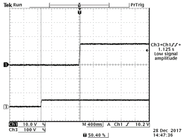
Figure 26. Startup from
