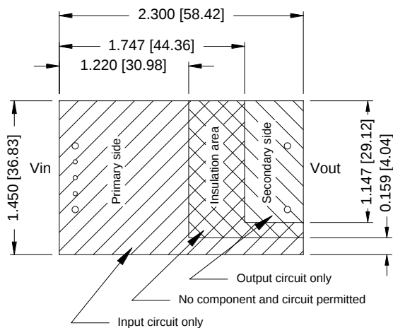
Figure 54. 0RQB-50Y15L/0 Recommended pad layout-1
