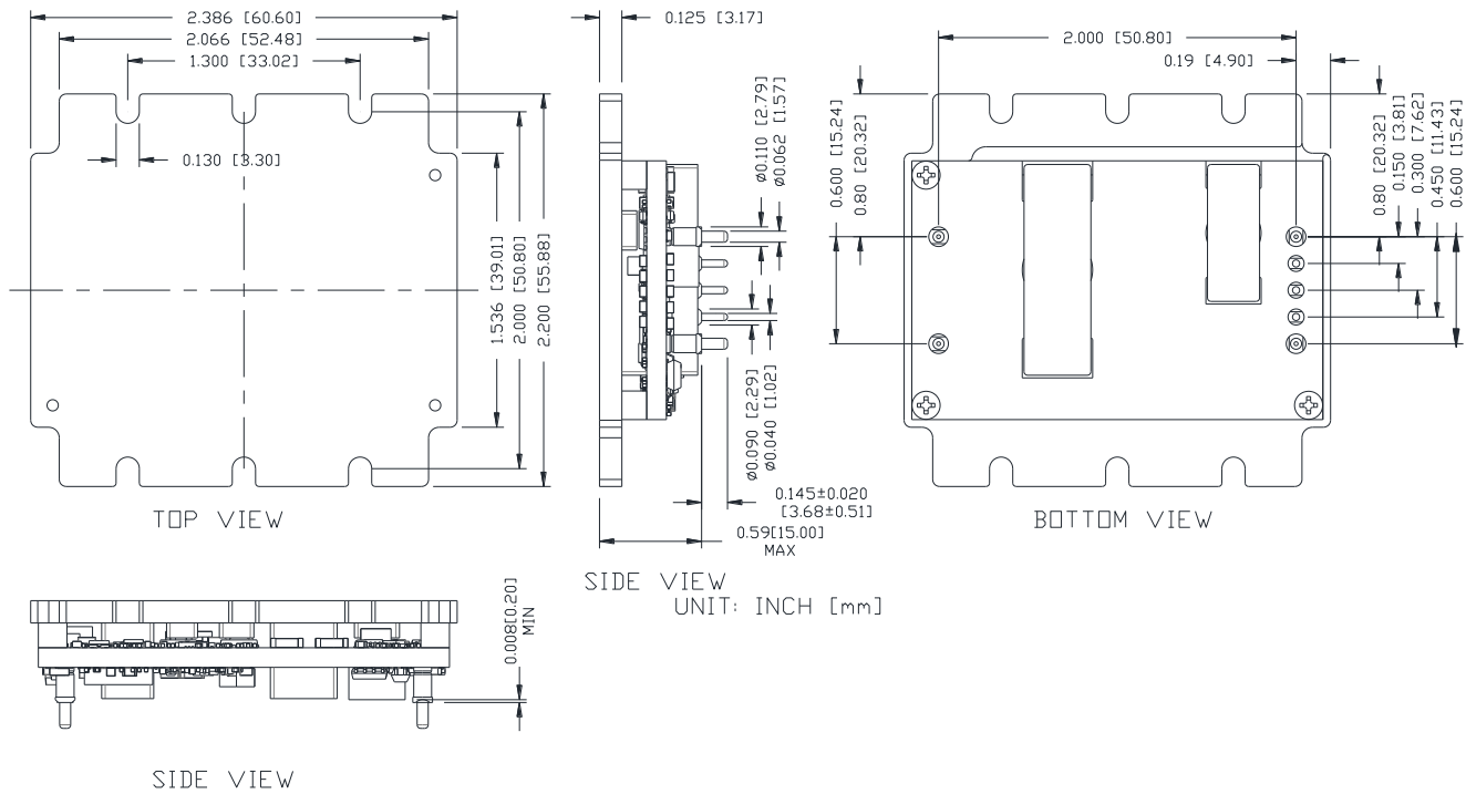
Figure 56. 0RQB-50Y15E/F Outline
