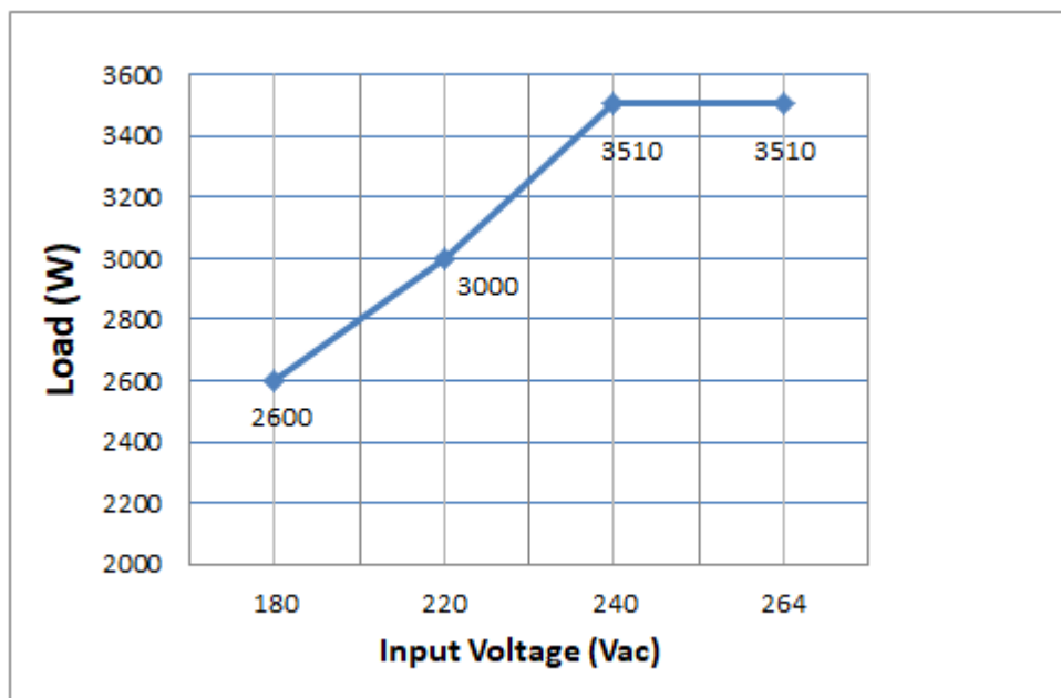
Figure 1. Power Derating Curve
