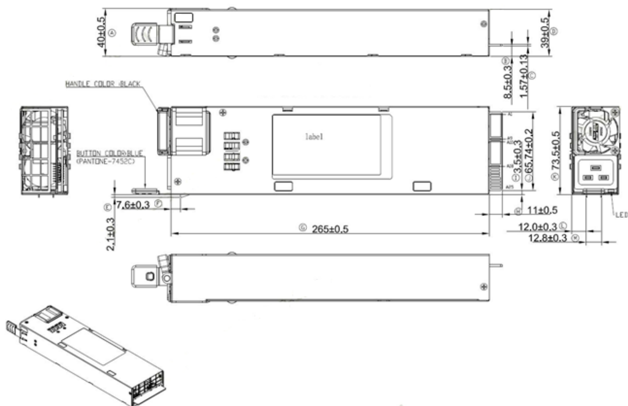
Figure 17. Mechanical Drawing
