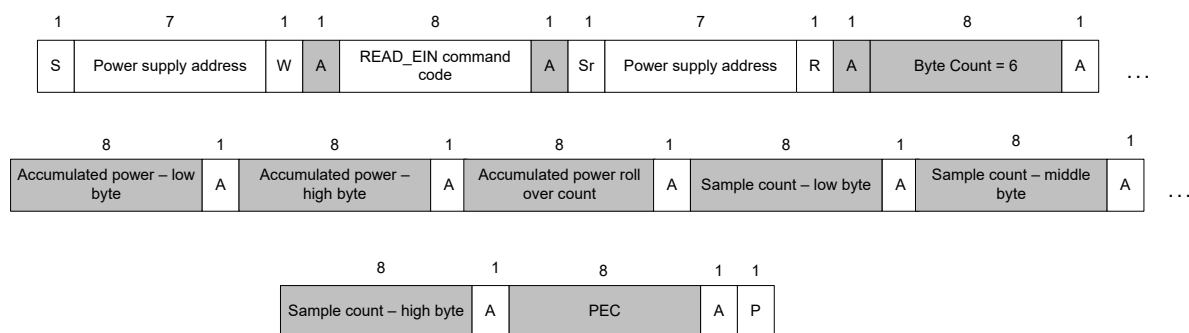
Figure 10. READ_EIN Command
