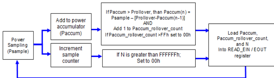
Figure 11. READ_EIN PSU Functional Diagram
