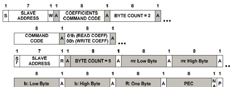
Figure 9. Retrieving Coefficients Using PEC
