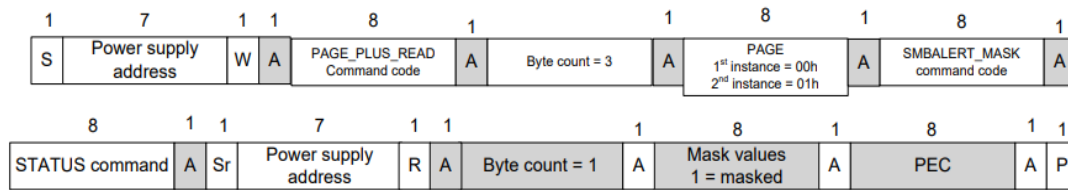
Figure 7. PAGE_PLUS_READ command.
