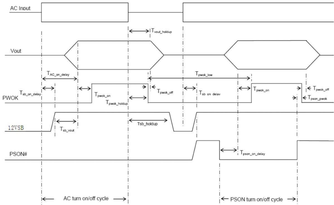
Figure 2. Signal Timing Sequence
