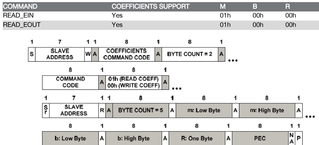
Figure 5. Retrieving Coefficients Using PEC
