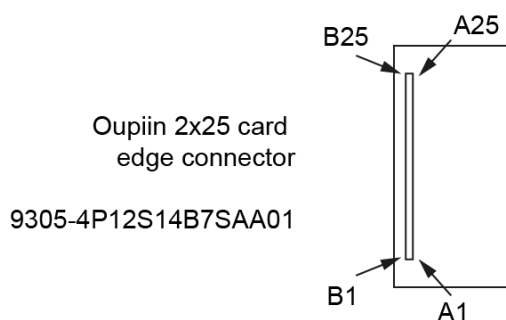
Figure 20. Back DC output golden finger port
