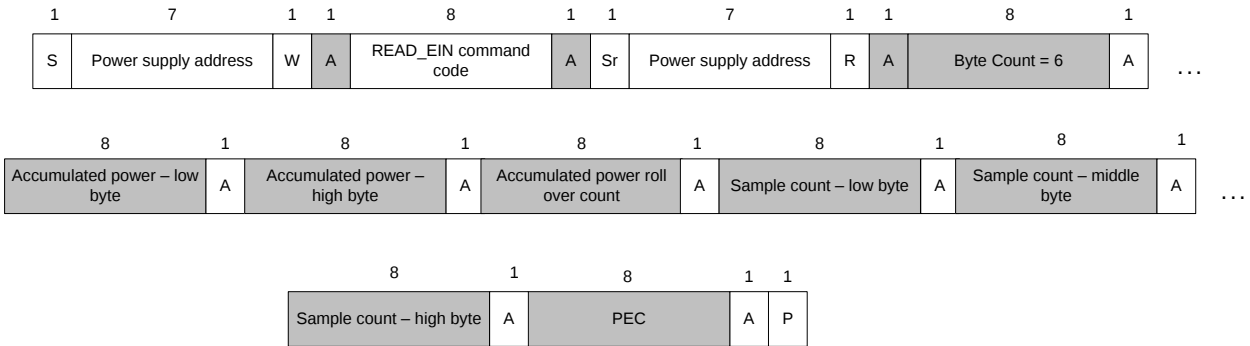
Figure 12. READ_EIN Command
