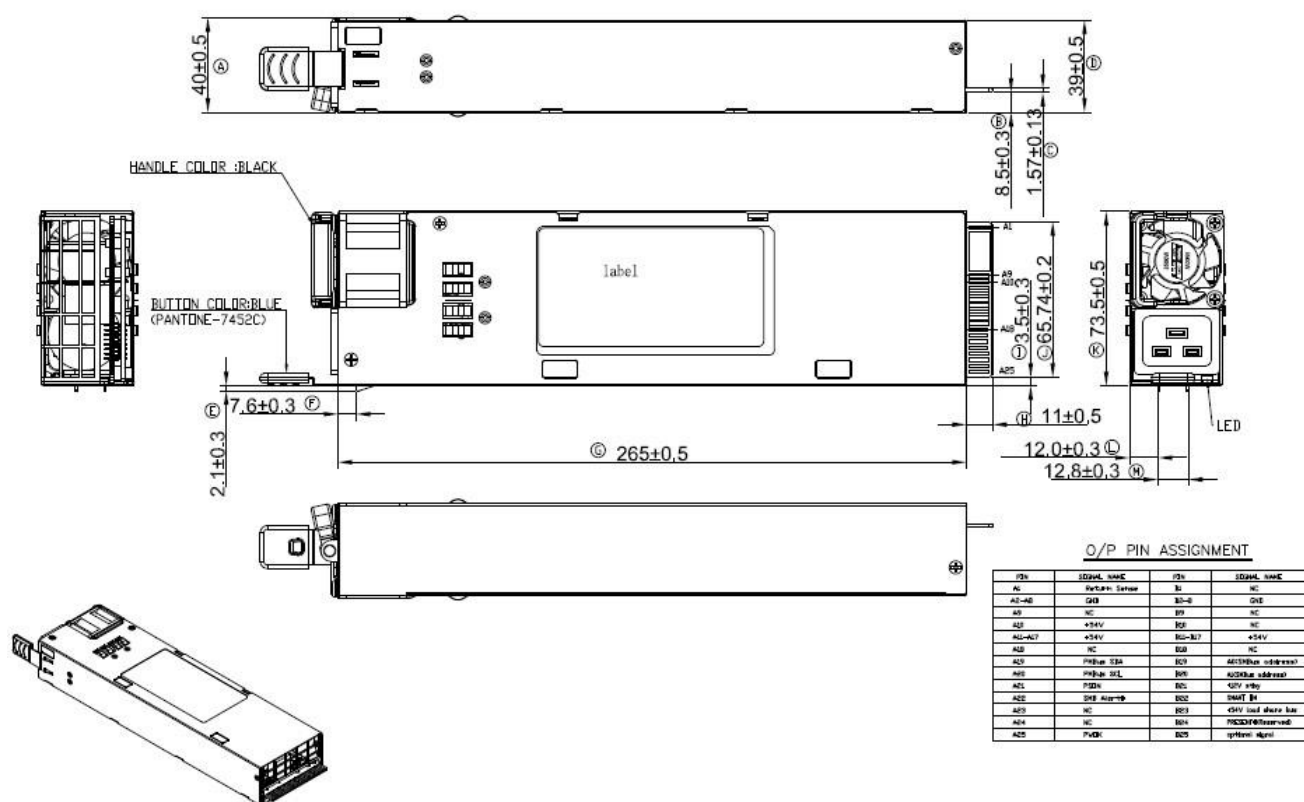
Figure 19. Mechanical Drawing
