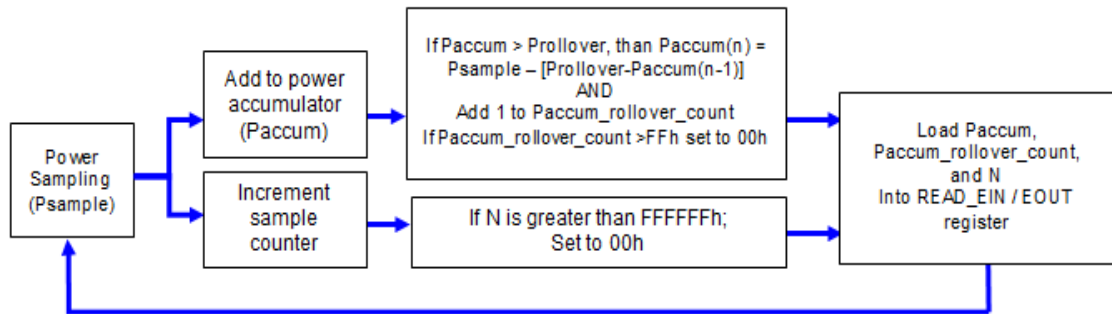
Figure 13. READ_EIN PSU Functional Diagram
