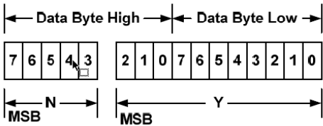
Figure 14. Linear Data Format Data Bytes
