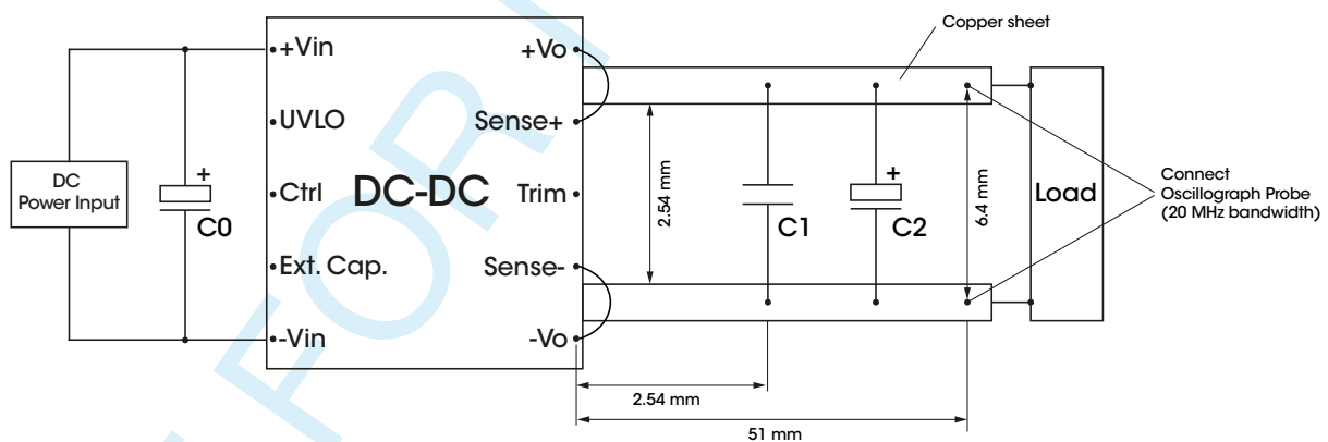
Figure 5. Recommended Test Circuit
