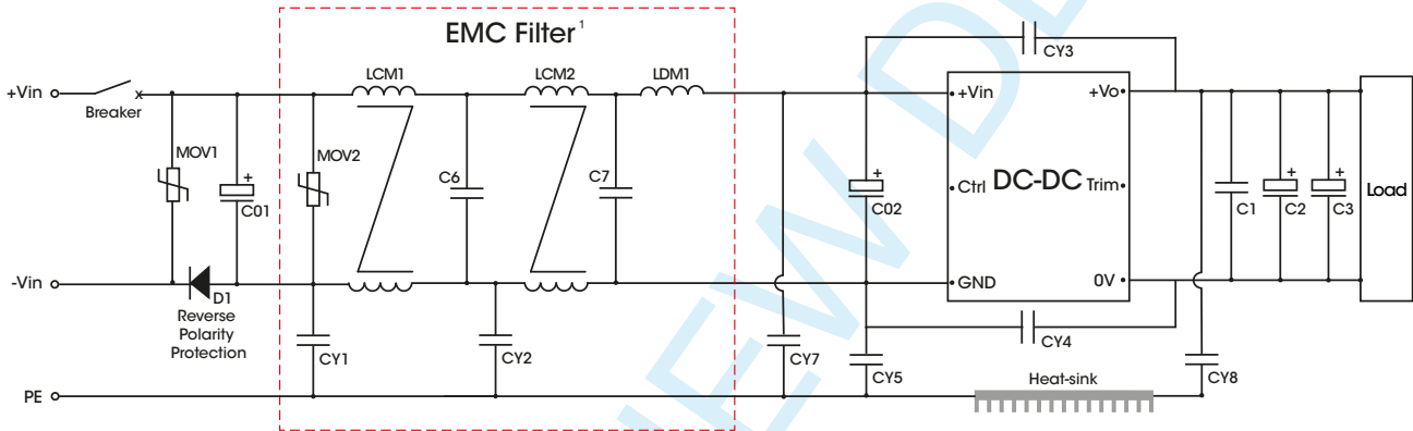
Figure 6. Recommended EMC Filtering with PE
