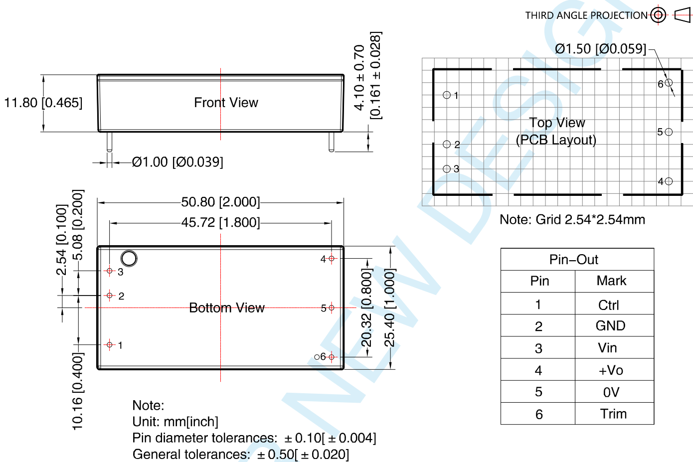
Figure 8. Mechanical Drawing of Standard Model
