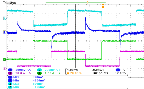
Figure 10. Load transient V 1 , V SB .0 to 50% full load (4ms/div) CH1: V1 (200mV~div) CH2: V SB (200mV~div) CH3: I1 (50A/div) CH4: I SB (1.5A/div)
