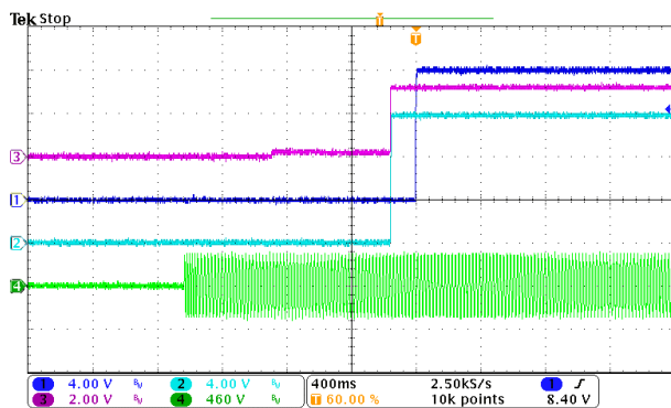
Figure 5. Turn-On AC Line 230VAC, full load (400ms/div)
