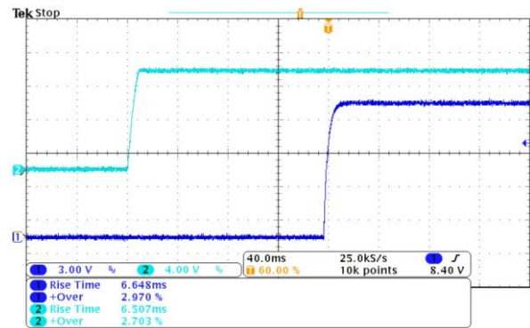
Figure 6. Turn-On AC Line 230VAC, no load (40ms/div)
