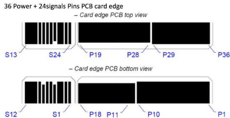
Figure 30. Output gold finger in PSU
