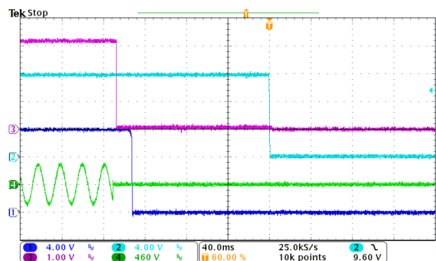
Figure 8. Turn-Off AC Line 230VAC, full load (40ms/div)
