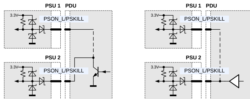
Figure 16. PSON_L/PSKILL connection
