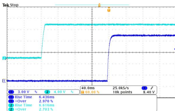
Figure 7. Turn-On AC Line 230VAC, full load (40ms/div)
