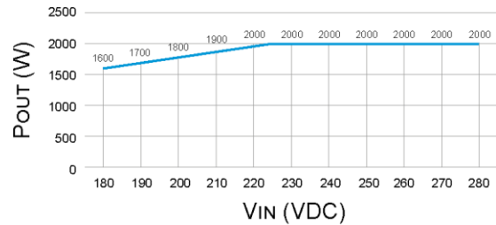
Figure 2. Power Derating Curve 2
