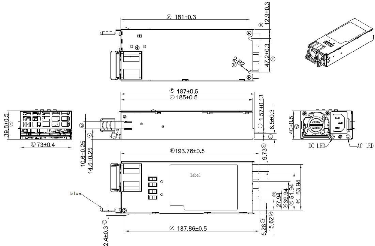
Figure 4. Mechanical Drawing
