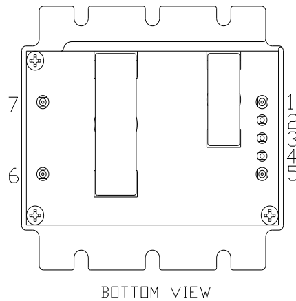
Figure 57. 0RQB-50Y48E/F Pins
