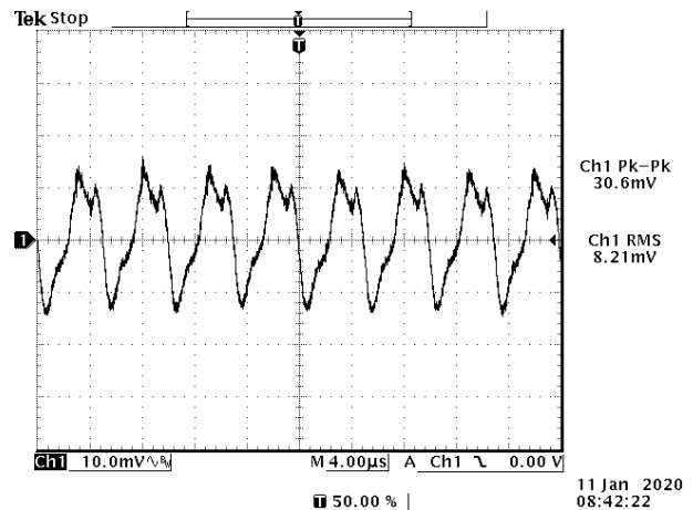
Figure 17. Ripple and noise, V_{in} = 110 \text{ Vdc} , 48 \text{ Vdc}/10.4 \text{ A} output @ T_a=25^\circ\text{C} with C_{ext} = 200 \mu\text{F}
