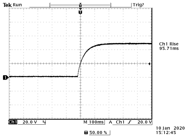
Figure 22. V_{in} = 48\text{ V} , I_o = 1.04\text{ A} , V_o = 48\text{ V} with C_{ext} = 200\text{ }\mu\text{F}
