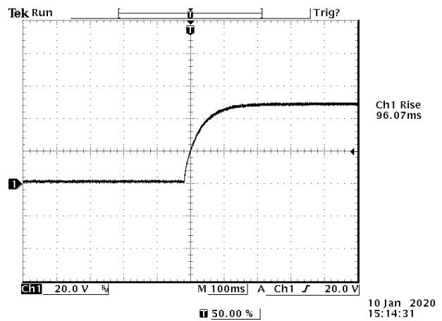
Figure 25. V_{in} = 110\text{ V} , I_o = 1.04\text{ A} , V_o = 48\text{ V} with C_{ext} = 1200\text{ }\mu\text{F}
