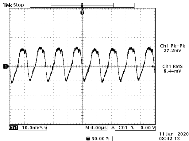
Figure 16. Ripple and noise, V_{in} = 48 \text{ Vdc} , 48 \text{ Vdc}/1.04 \text{ A} output @ T_a=25^\circ\text{C} with C_{ext} = 200 \mu\text{F}
