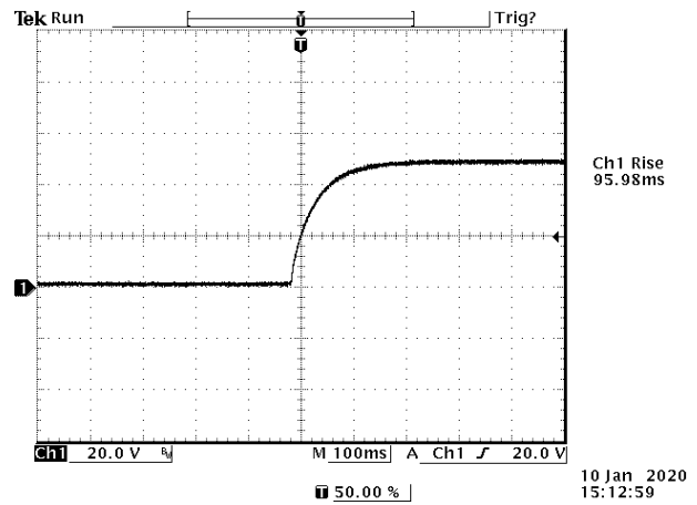
Figure 23. V_{in} = 110\text{ V} , I_o = 1.04\text{ A} , V_o = 48\text{ V} with C_{ext} = 200\text{ }\mu\text{F}
