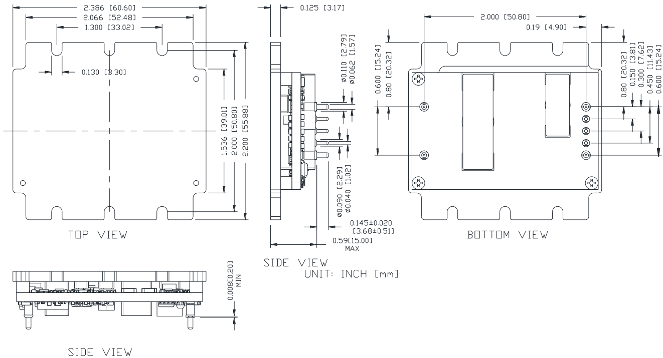
Figure 56. 0RQB-50Y48E/F Outline
