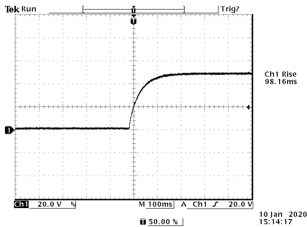
Figure 24. V_{in} = 48\text{ V} , I_o = 1.04\text{ A} , V_o = 48\text{ V} with C_{ext} = 1200\text{ }\mu\text{F}
