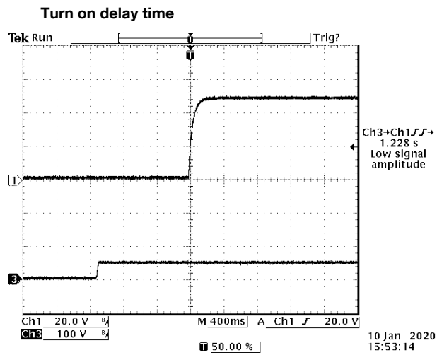
Figure 26. Startup from Vin
