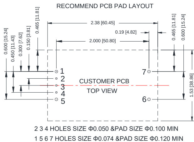
Figure 55. ORQB-50Y48L/0 Recommended pad layout-2
