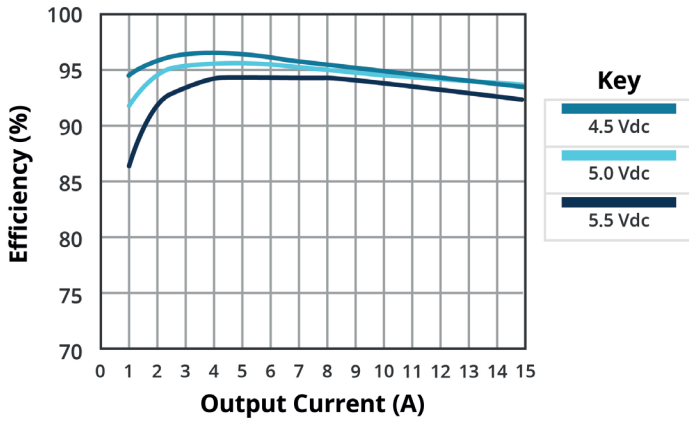
EFFICIENCY VS OUTPUT CURRENT VPOL15A-5-SIP (Vo = 3.3 Vdc)
