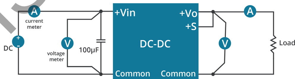
Figure 4 VPOL10A-12W-SIP Series Test Setup
