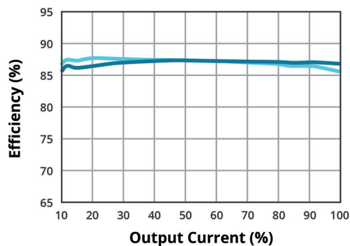
EFFICIENCY VS OUTPUT LOAD (VOF-50E-15)
