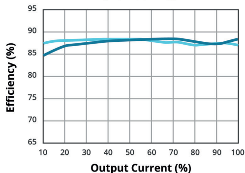
EFFICIENCY VS OUTPUT LOAD (VOF-50E-36)
