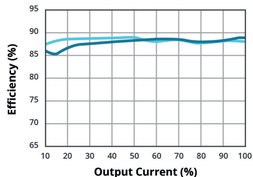
EFFICIENCY VS OUTPUT LOAD (VOF-50E-48)
