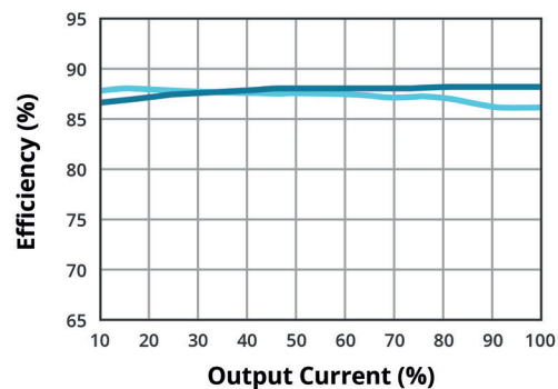
EFFICIENCY VS OUTPUT LOAD (VOF-50E-24)
