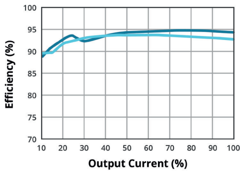
EFFICIENCY VS OUTPUT LOAD (VOF-500B-24)
