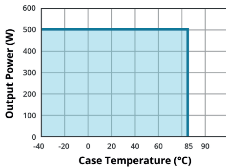
CASE TEMPERATURE DERATING CURVE (T c )
