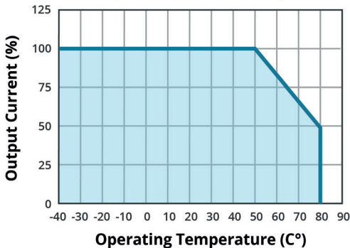
TEMPERATURE DERATING CURVE (natural convection)
