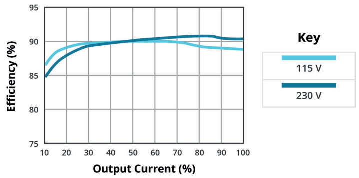
EFFICIENCY VS OUTPUT LOAD (VOF-36E-24)
