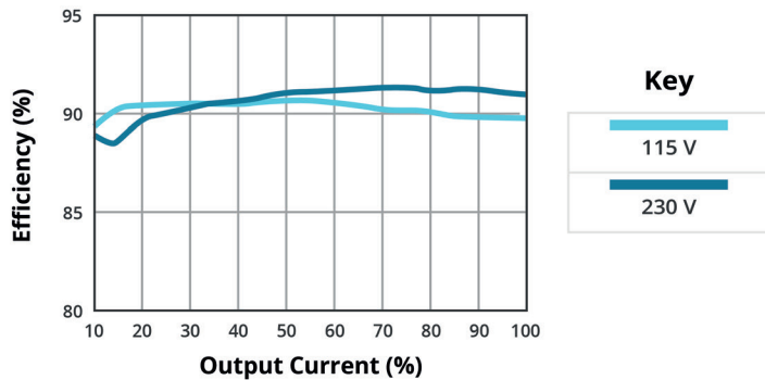
EFFICIENCY VS OUTPUT LOAD (VGS-70E-36)
