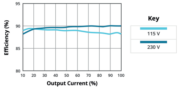
EFFICIENCY VS OUTPUT LOAD (VGS-70E-48)
