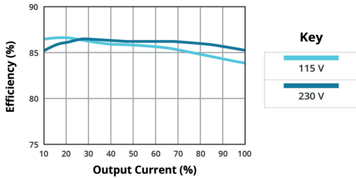
EFFICIENCY VS OUTPUT LOAD (VGS-70E-15)
