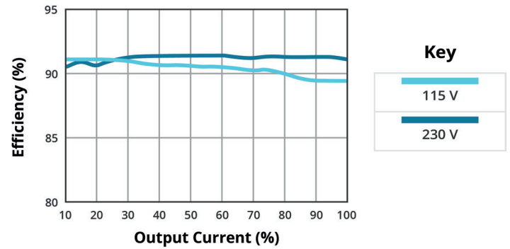
EFFICIENCY VS OUTPUT LOAD (VGS-70E-24)
