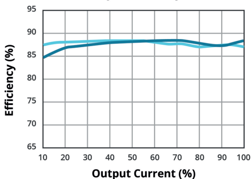
EFFICIENCY VS OUTPUT LOAD (VGS-50E-15)
