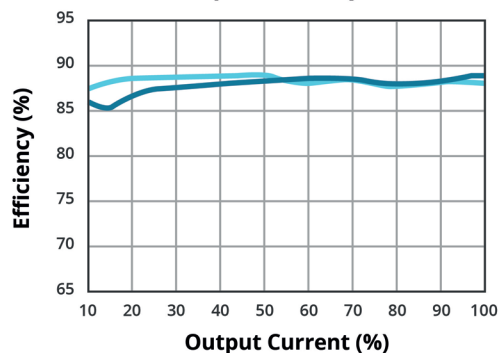
EFFICIENCY VS OUTPUT LOAD (VGS-50E-24)
