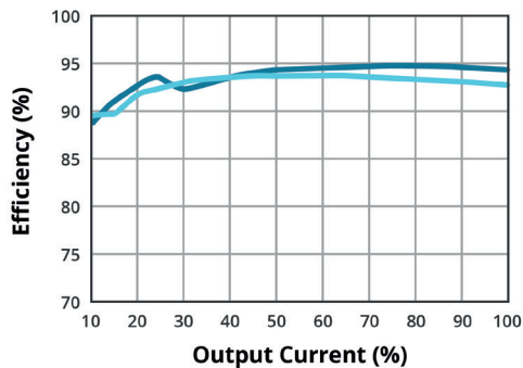
EFFICIENCY VS OUTPUT LOAD (VGS-500B-24)
