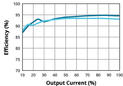
EFFICIENCY VS OUTPUT LOAD (VGS-500B-28)
