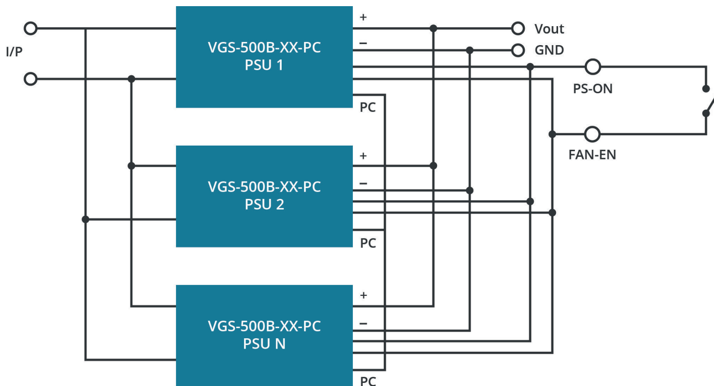
Figure 4 Connection diagram for parallel operation and current sharing
