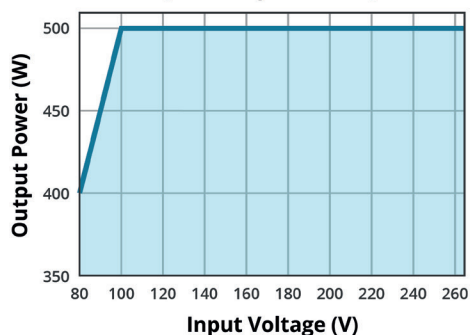
INPUT VOLTAGE DERATING CURVE (21 CFM forced air)
