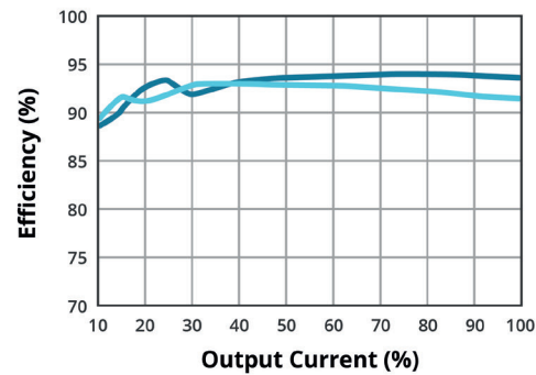
EFFICIENCY VS OUTPUT LOAD (VGS-500B-18)
