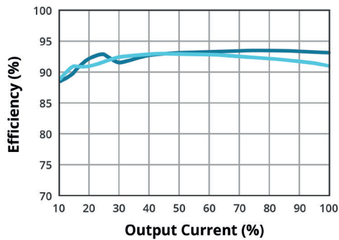
EFFICIENCY VS OUTPUT LOAD (VGS-500B-12)
