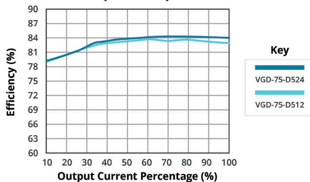
EFFICIENCY VS OUTPUT LOAD (at 230 Vac)
